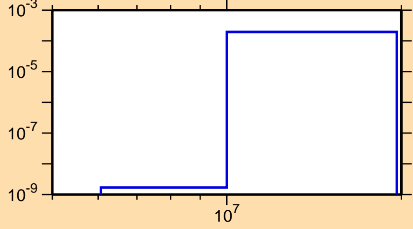
\sigma vs. E for ^{256}\text{Md}(n,t)
