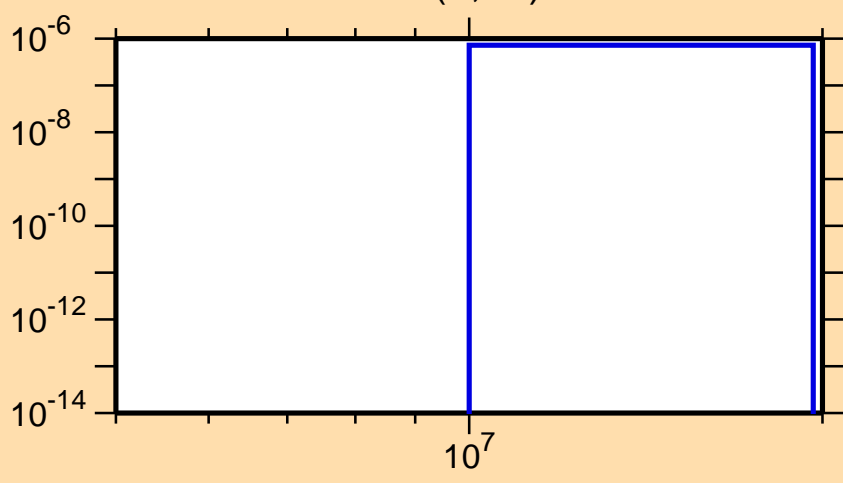
\sigma vs. E for ^{256}\text{Md}(n,\text{nd})
