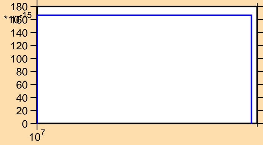
\sigma vs. E for ^{256}\text{Md} (mt 11)
