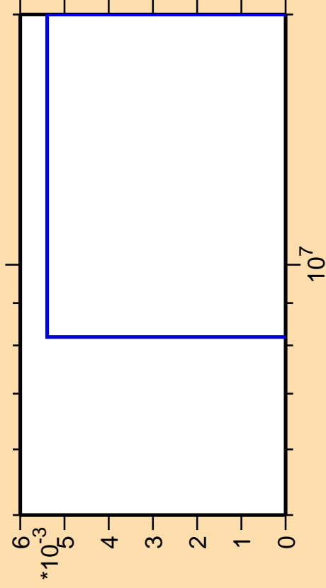
\Delta\sigma/\sigma vs. E for ^{256}\text{Md}(\text{mt } 34)
