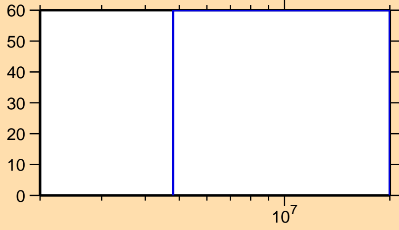
\Delta\sigma/\sigma vs. E for ^{256}\text{Md}(n,\text{inel.})
