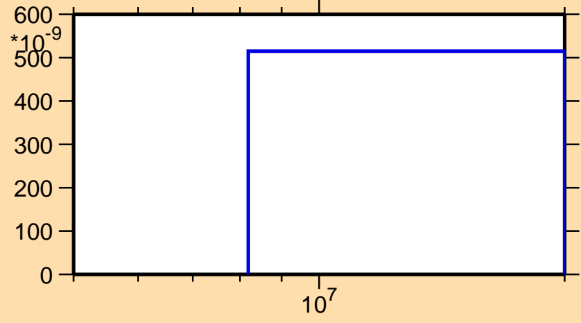
\sigma vs. E for ^{256}\text{Md}(n,nt)
