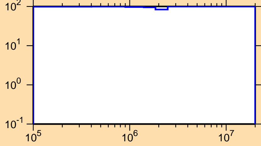
\Delta\sigma/\sigma vs. E for ^{256}\text{Md}(n,n_1)
