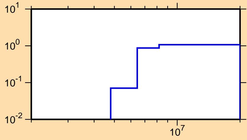
\sigma vs. E for ^{256}\text{Md}(n,2n)
