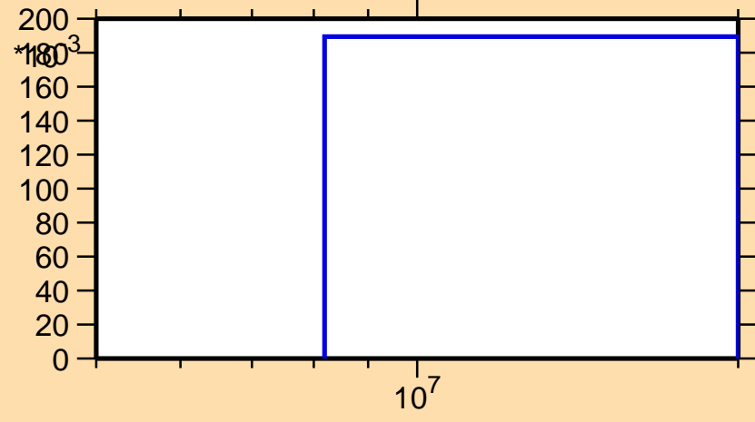
\sigma vs. E for ^{256}\text{Md}(n,3n)
