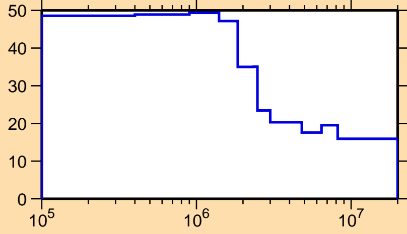
\Delta\sigma/\sigma vs. E for ^{256}\text{Md}(n,n\text{onel.})
