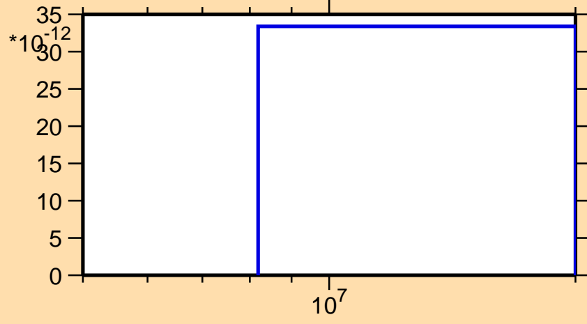
\sigma vs. E for ^{256}\text{Md}(n,3n\alpha)
