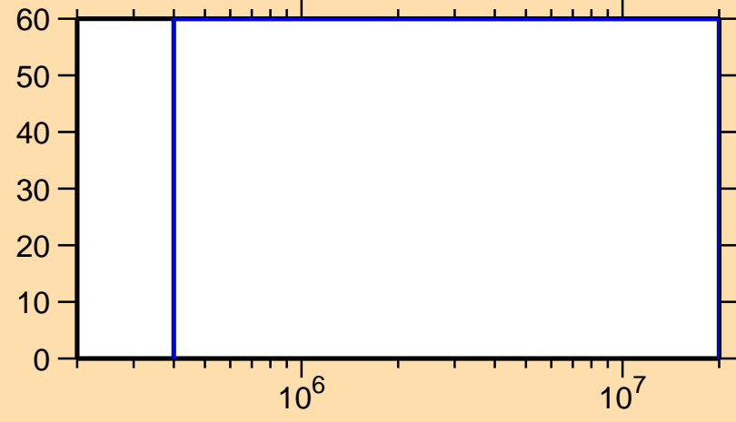
\Delta\sigma/\sigma vs. E for ^{256}\text{Md}(n,ncont.)
