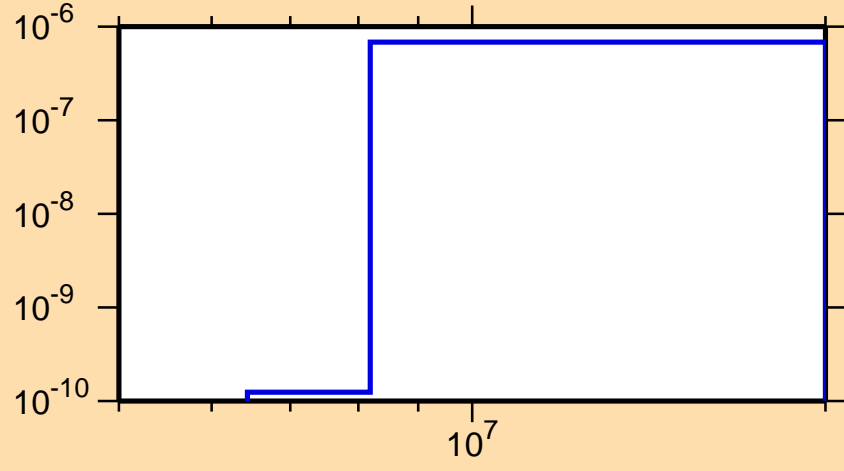
\sigma vs. E for ^{256}\text{Md}(n,2n\alpha)
