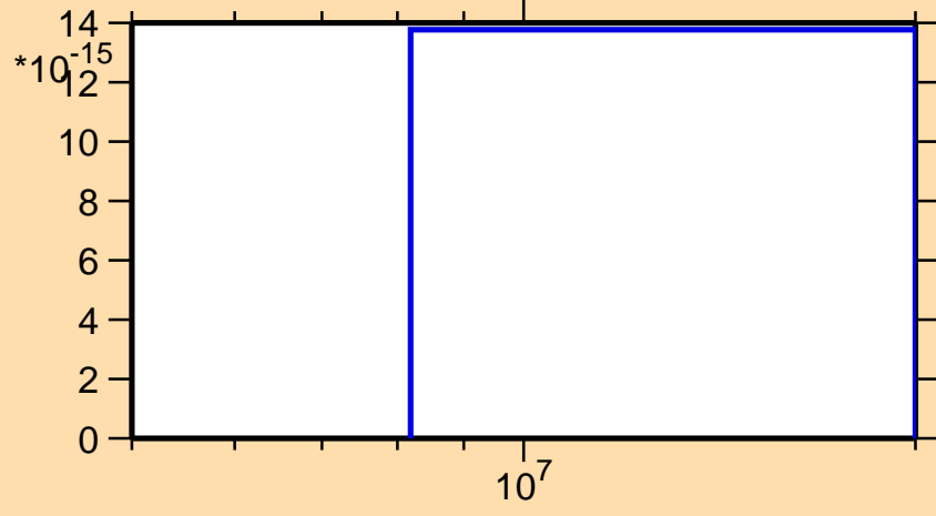
\sigma vs. E for ^{256}\text{Md} (mt 45)
