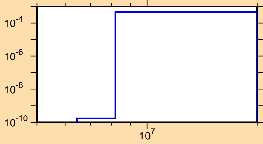
\sigma vs. E for ^{256}\text{Md}(n,d)
