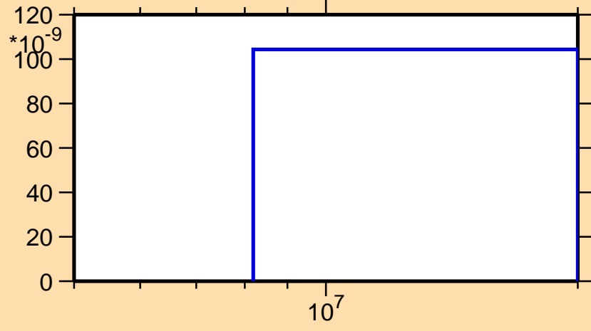
\sigma vs. E for ^{256}\text{Md}(n,2np)
