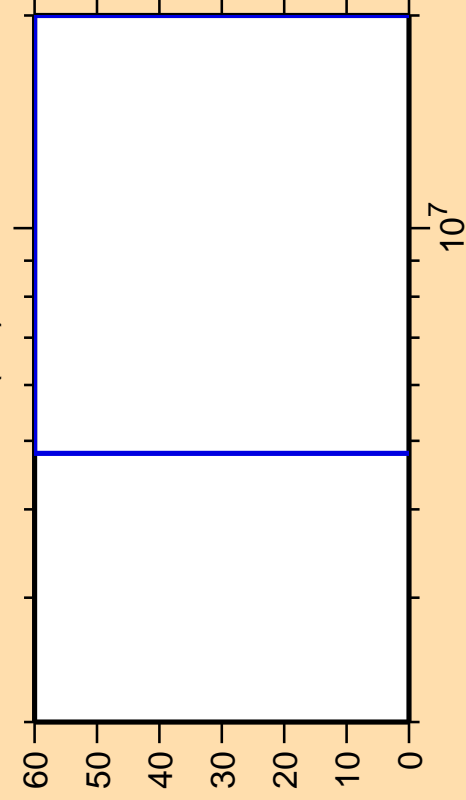
\Delta\sigma/\sigma vs. E for ^{256}\text{Md}(n,f)
