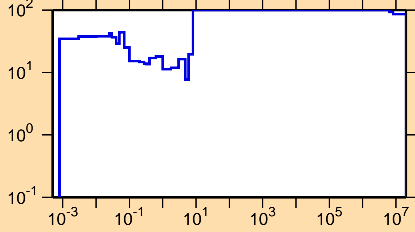
\Delta\sigma/\sigma vs. E for ^{256}\text{Md}(n,f)
