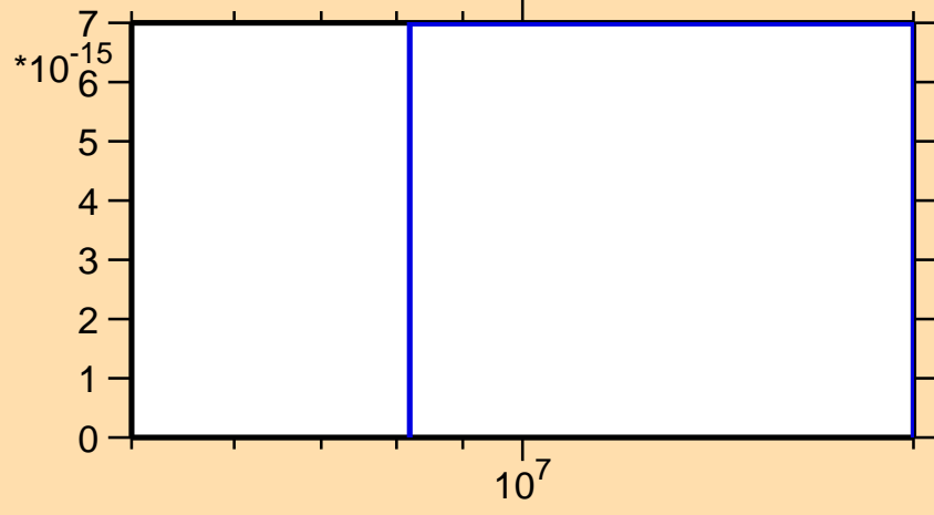
\sigma vs. E for ^{256}\text{Md}(\text{mt } 34)
