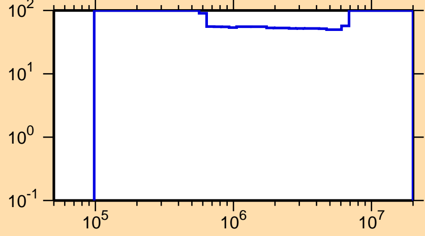
\Delta\sigma/\sigma vs. E for ^{257}\text{Md}(n,\text{inel.})
