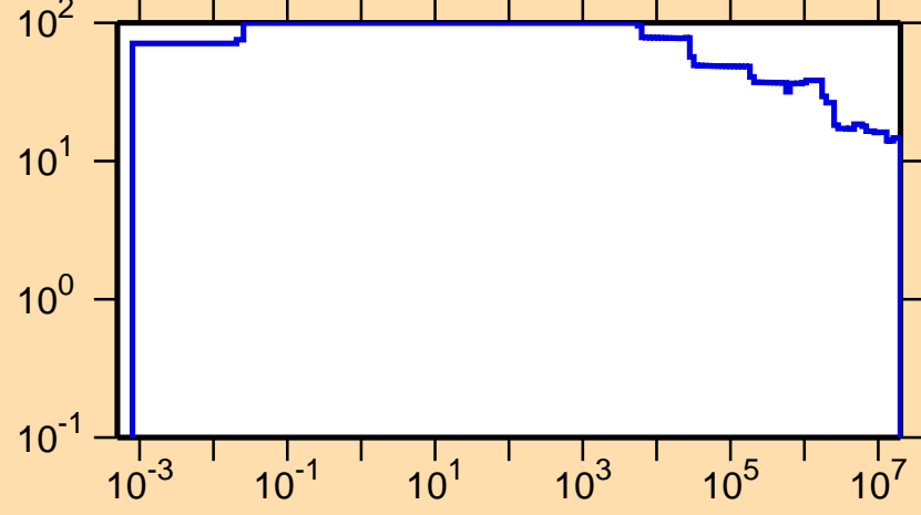
\Delta\sigma/\sigma vs. E for ^{257}\text{Md}(n,\text{nonel.})
