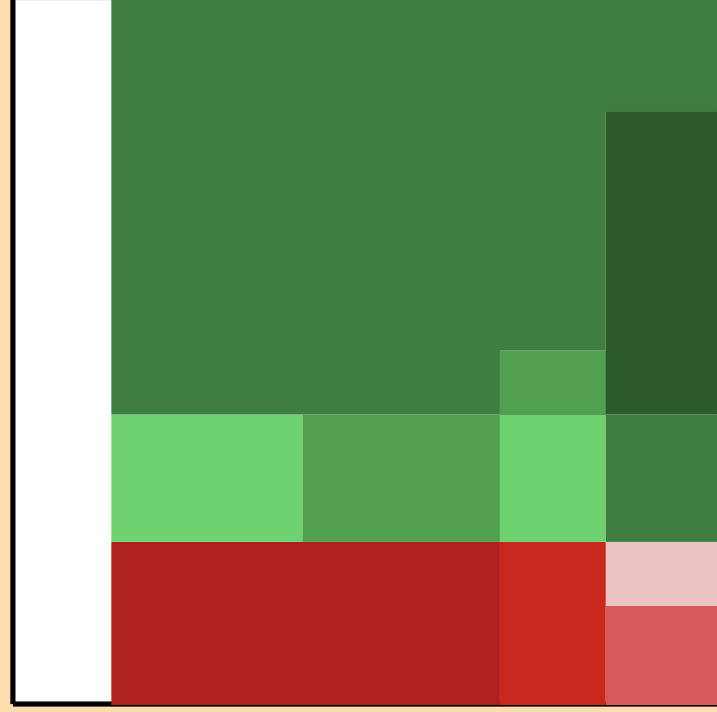
\Delta\sigma/\sigma vs. E for ^{257}\text{Md}(n,2n)
