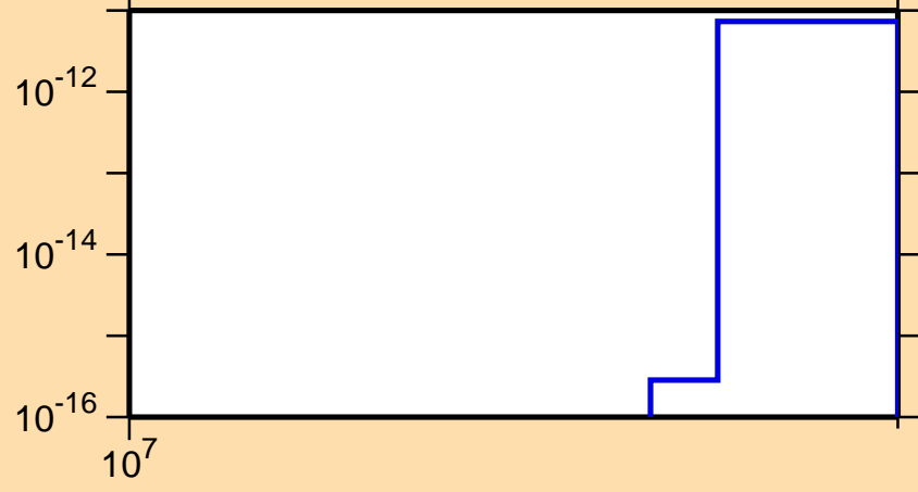
\sigma vs. E for ^{257}\text{Md} (mt 11)
