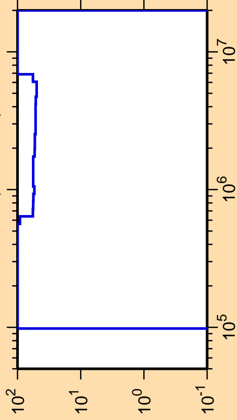
\Delta\sigma/\sigma vs. E for ^{257}\text{Md}(n,\text{ncont.})
