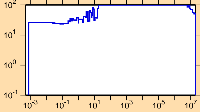
\Delta\sigma/\sigma vs. E for ^{257}\text{Md}(n,f)
