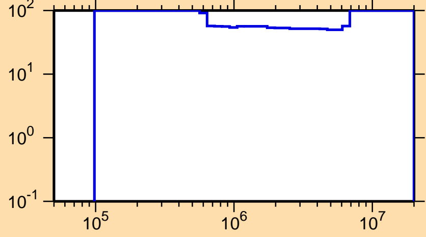
\Delta\sigma/\sigma vs. E for ^{257}\text{Md}(n,n\text{cont.})
