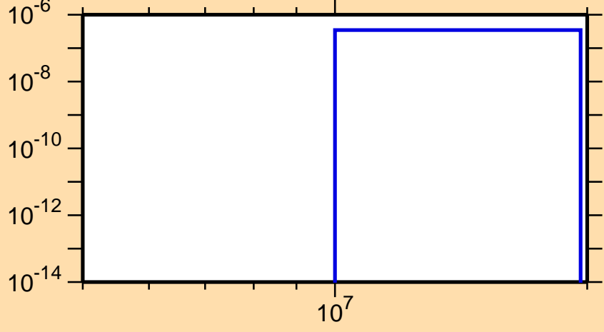
\sigma vs. E for ^{257}\text{Md}(n,nt)
