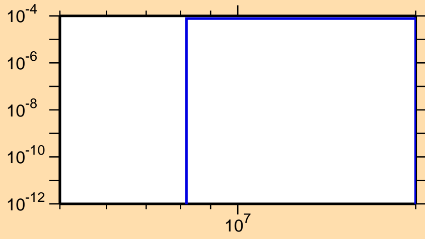
\sigma vs. E for ^{257}\text{Md}(n,t)
