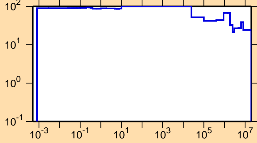
\Delta\sigma/\sigma vs. E for ^{257}\text{Md}(n,\text{el.})
