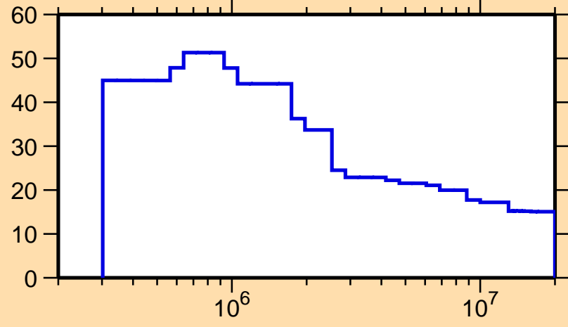
\Delta\sigma/\sigma vs. E for ^{258}\text{Md}(n,n\text{onel.})
