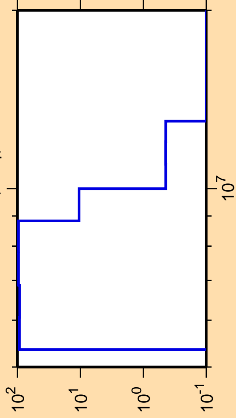
\Delta\sigma/\sigma vs. E for ^{258}\text{Md}(n,n_1)
