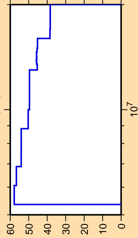
\Delta\sigma/\sigma vs. E for ^{258}\text{Md}(n,f)
