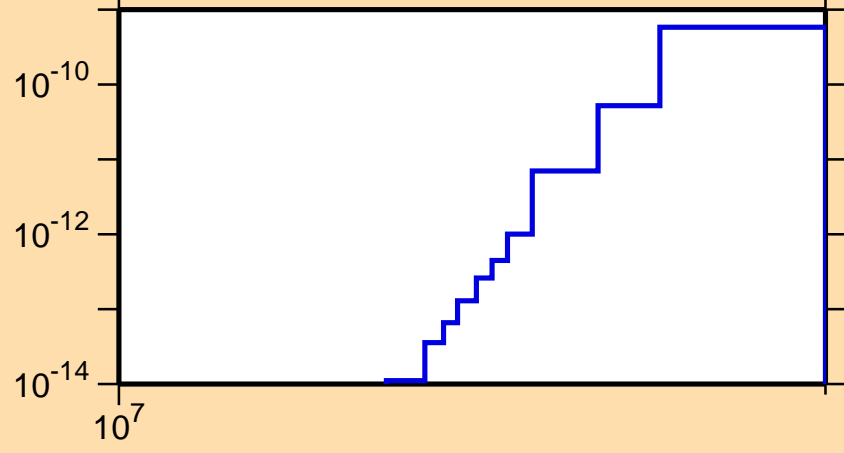
\sigma vs. E for ^{258}\text{Md}(n,\text{He}3)
