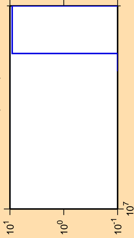
\Delta\sigma/\sigma vs. E for ^{258}\text{Md}(\text{mt } 11)
