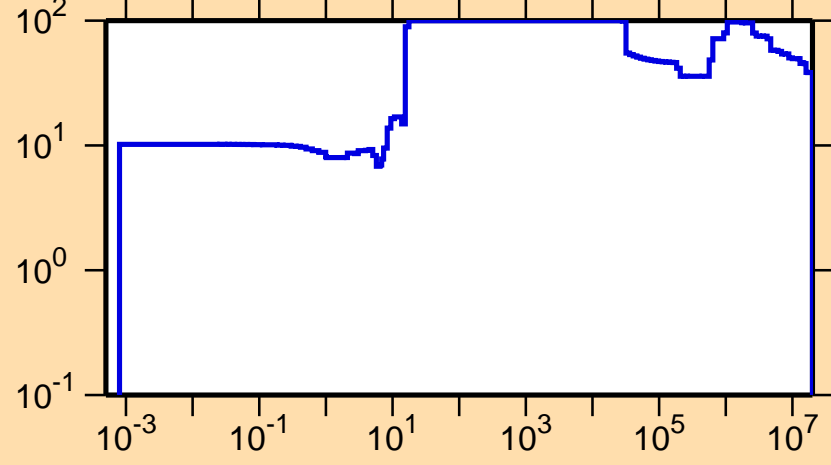
\Delta\sigma/\sigma vs. E for ^{258}\text{Md}(n,f)
