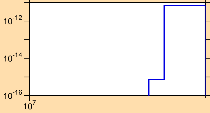
\sigma vs. E for ^{258}\text{Md}(\text{mt } 11)
