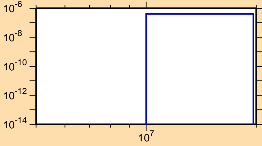
\sigma vs. E for ^{258}\text{Md}(n,\text{nd})
