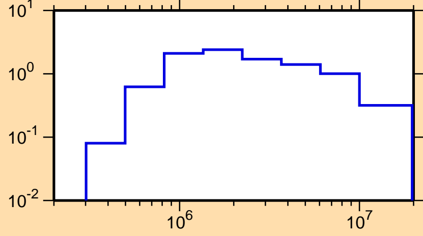
\sigma vs. E for ^{258}\text{Md}(n,n\text{cont.})
