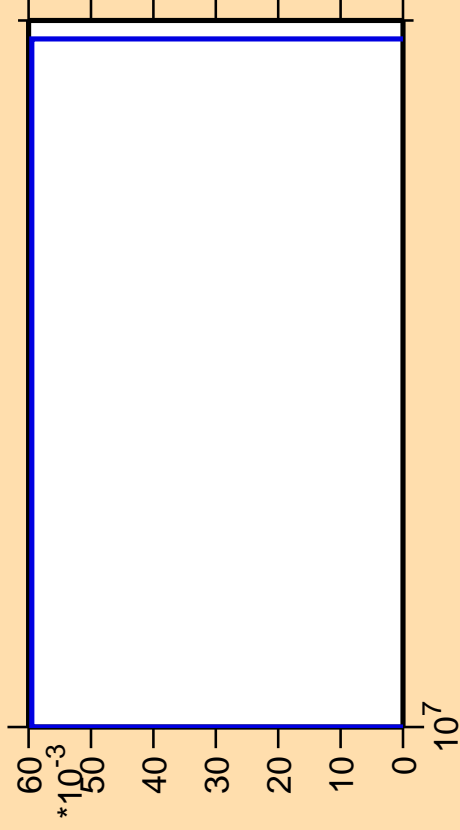
\Delta\sigma/\sigma vs. E for ^{258}\text{Md} (mt 11)
