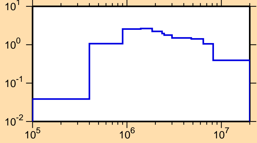
\sigma vs. E for ^{258}\text{Md}(n,\text{inel.})
