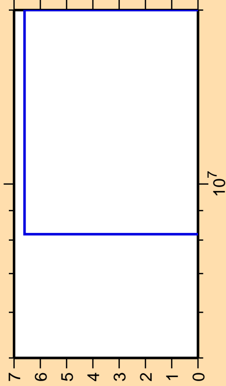
\Delta\sigma/\sigma vs. E for ^{258}\text{Md}(n,3n\alpha)
