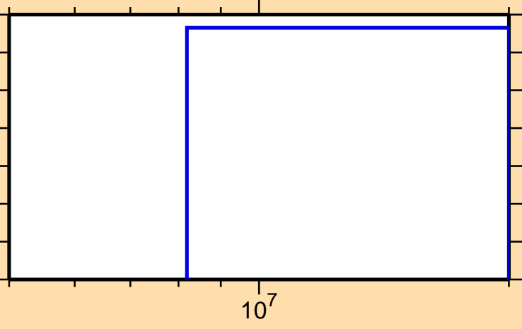
\sigma vs. E for ^{258}\text{Md}(n,\text{nd})
