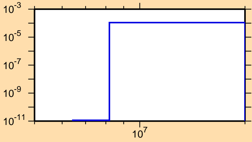
\sigma vs. E for ^{258}\text{Md}(n,t)
