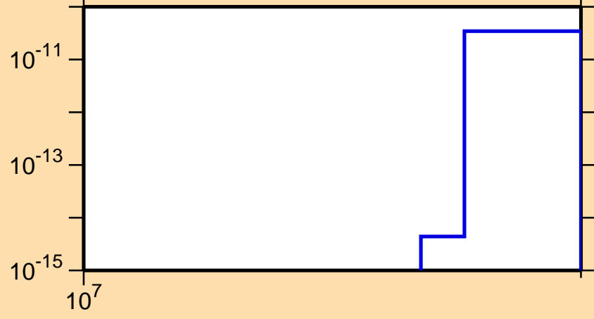
\sigma vs. E for ^{258}\text{Md} (mt 11)
