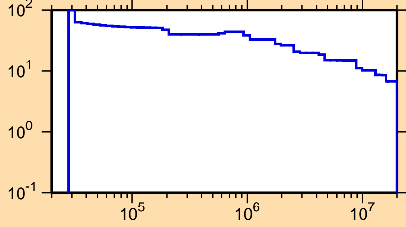
\Delta\sigma/\sigma vs. E for ^{258}\text{Md}(n,\text{nonel.})
