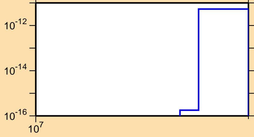
\sigma vs. E for ^{258}\text{Md} (mt 42)
