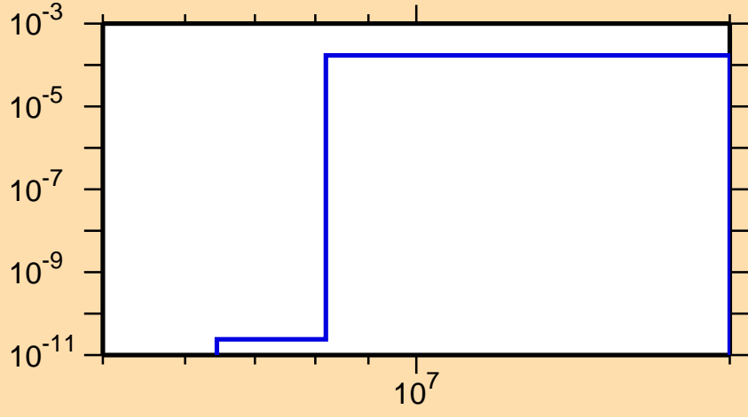
\sigma vs. E for ^{258}\text{Md}(n,d)
