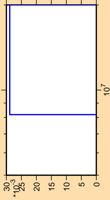
\Delta\sigma/\sigma vs. E for ^{258}\text{Md}(\text{mt } 34)
