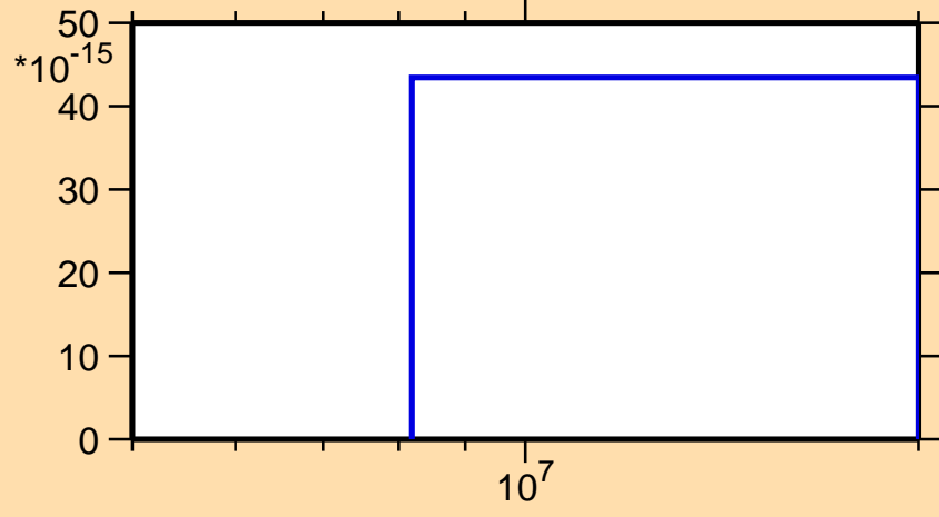
\sigma vs. E for ^{258}\text{Md} (mt 42)
