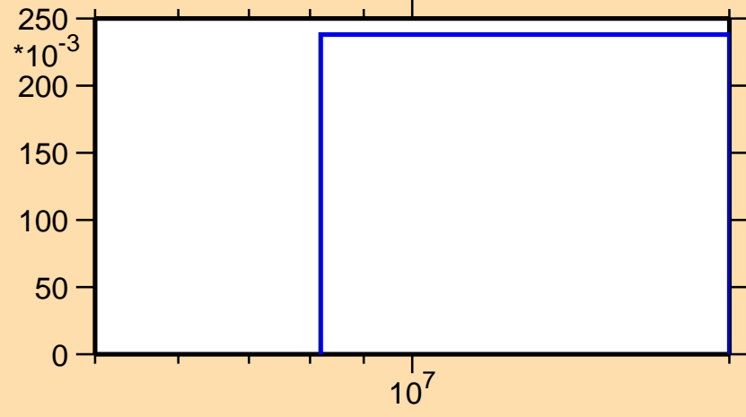
\sigma vs. E for ^{258}\text{Md}(n,3n)
