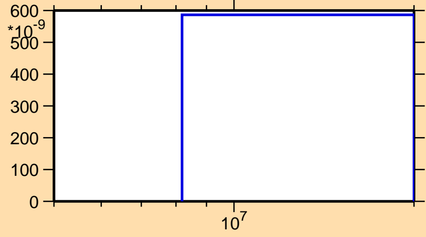
\sigma vs. E for ^{258}\text{Md}(n,nt)
