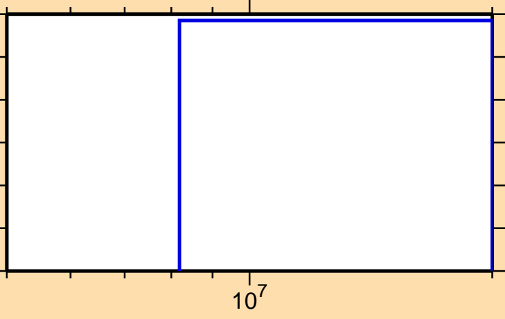
\sigma vs. E for ^{258}\text{Md}(n,\text{nd})
