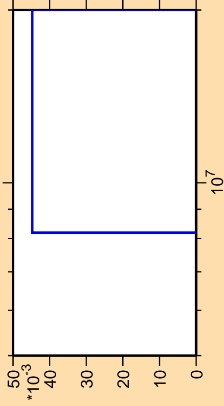
\Delta\sigma/\sigma vs. E for ^{258}\text{Md} (mt 42)
