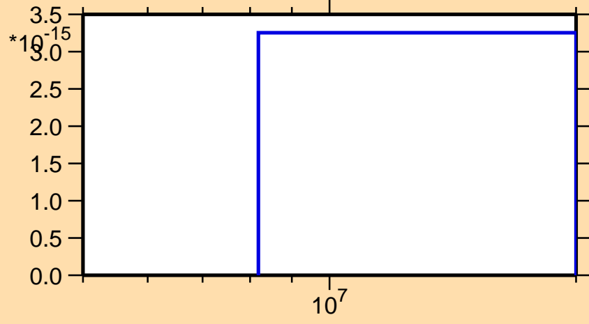
\sigma vs. E for ^{258}\text{Md}(\text{mt } 34)
