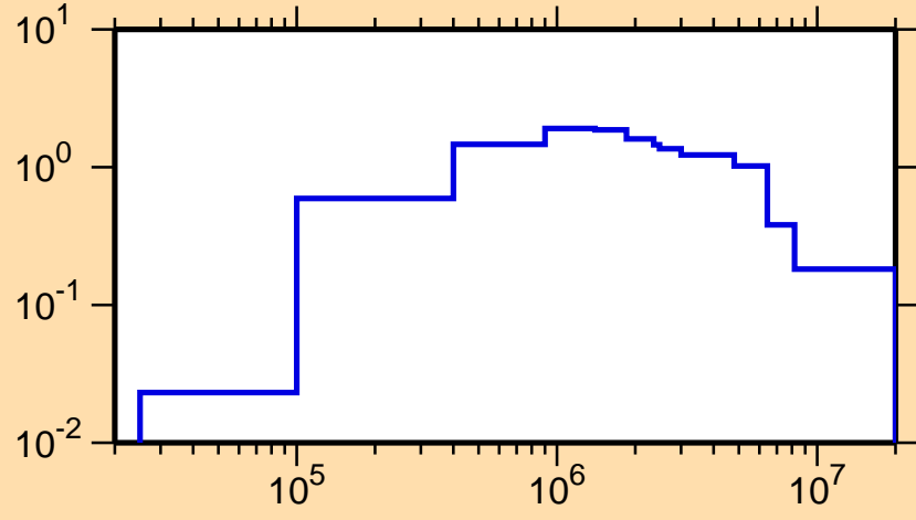
\sigma vs. E for ^{258}\text{Md}(n,n\text{cont.})
