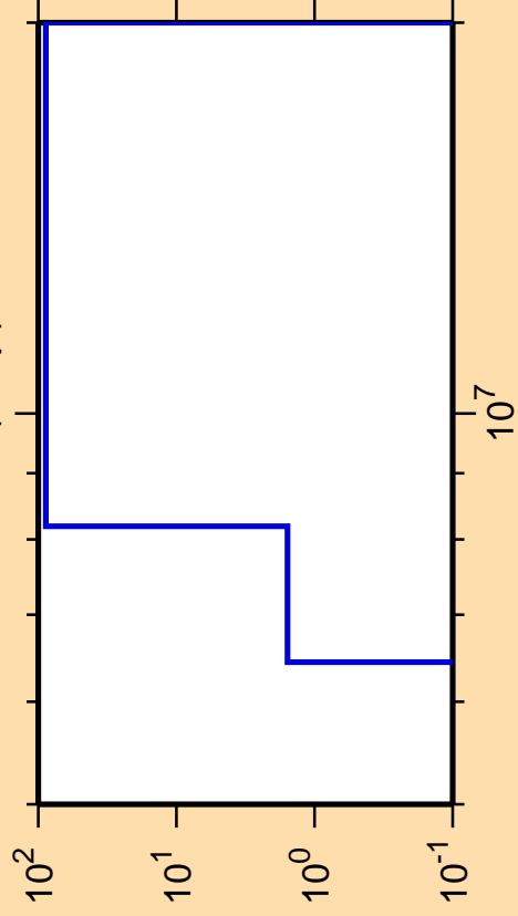
\Delta\sigma/\sigma vs. E for ^{258}\text{Md}(n,np)
