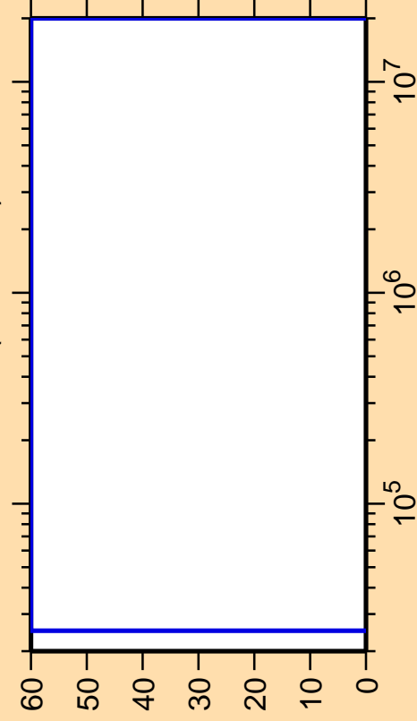
\Delta\sigma/\sigma vs. E for ^{258}\text{Md}(n,\text{ncont.})
