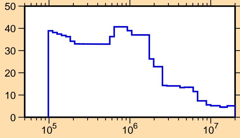
\Delta\sigma/\sigma vs. E for ^{259}\text{Md}(n,\text{nonel.})
