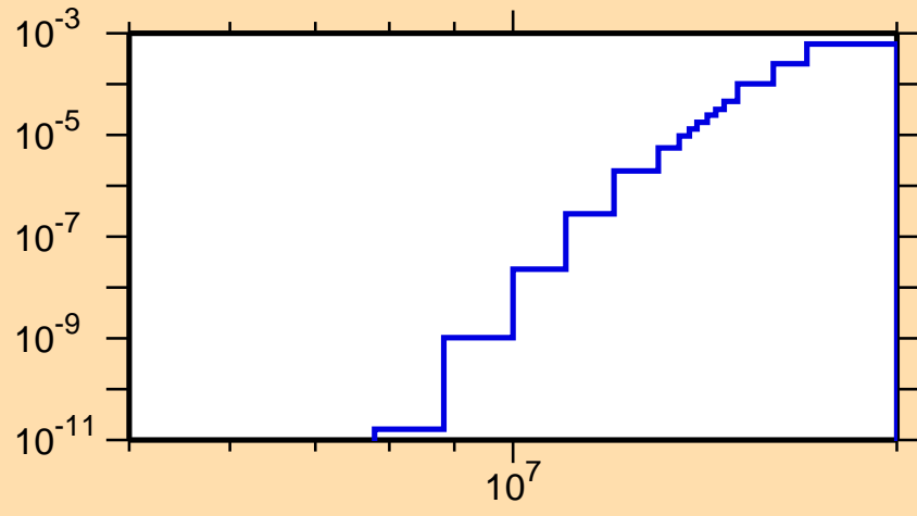
\sigma vs. E for ^{259}\text{Md}(n,np)
