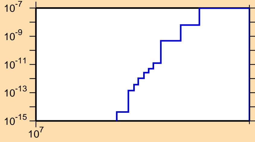
\sigma vs. E for ^{259}\text{Md}(n,2np)
