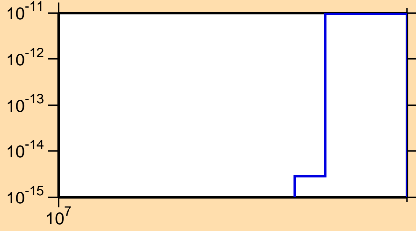
\sigma vs. E for ^{259}\text{Md} (mt 11)
