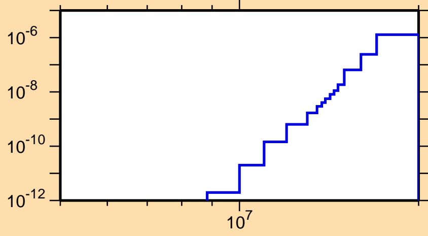
\sigma vs. E for ^{259}\text{Md}(n,2n\alpha)
