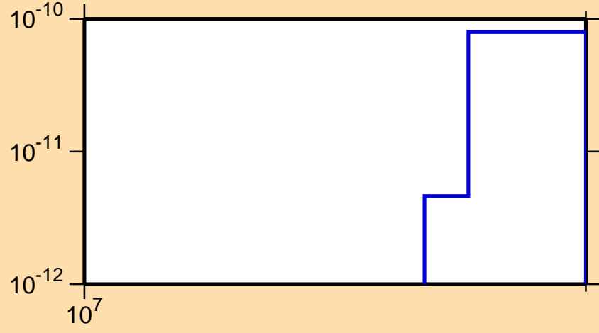
\sigma vs. E for ^{259}\text{Md}(n,\text{He}3)
