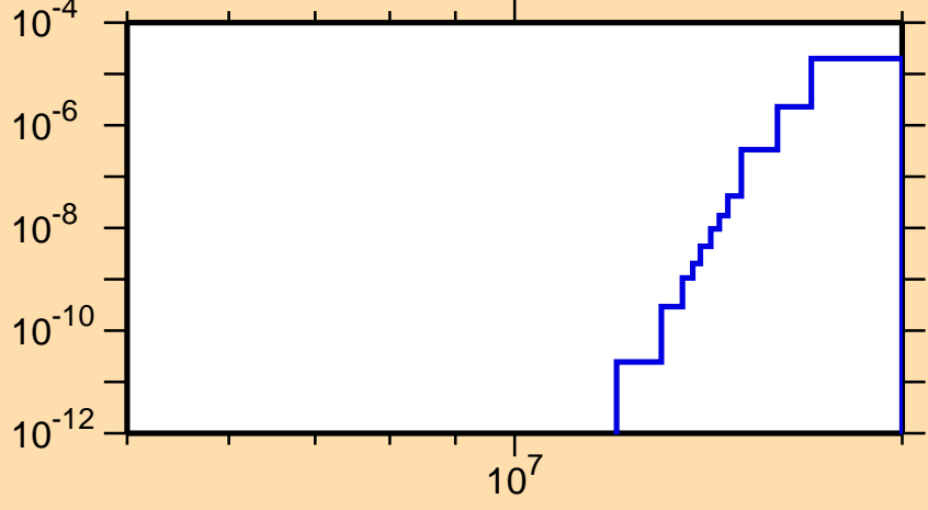
\sigma vs. E for ^{259}\text{Md}(n,nt)
