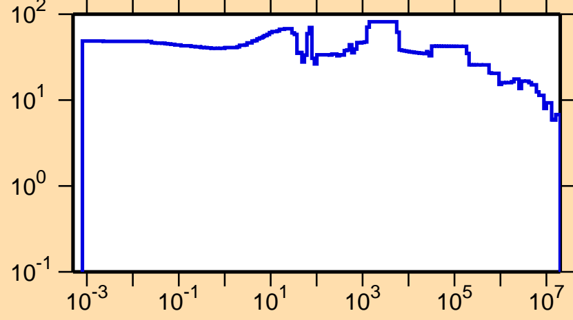
\Delta\sigma/\sigma vs. E for ^{259}\text{Md}(n,\text{tot.})
