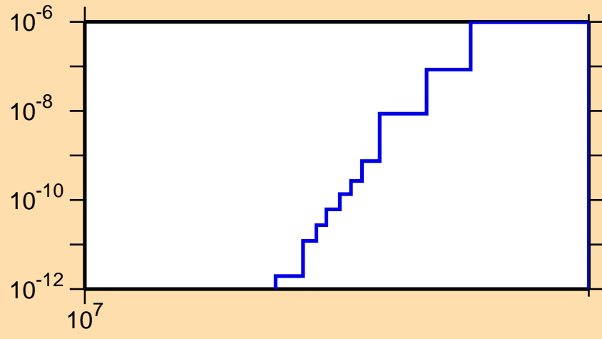
\sigma vs. E for ^{259}\text{Md}(n,\text{nd})
