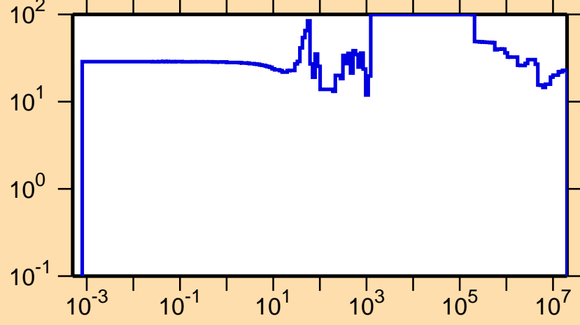
\Delta\sigma/\sigma vs. E for ^{259}\text{Md}(n,f)
