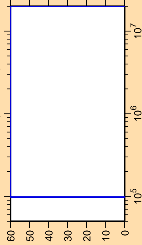
\Delta\sigma/\sigma vs. E for ^{259}\text{Md}(n,\text{ncont.})
