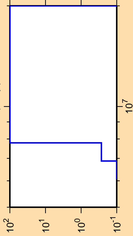
\Delta\sigma/\sigma vs. E for ^{259}\text{Md}(n,np)
