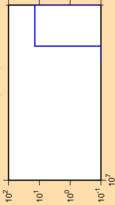
\Delta\sigma/\sigma vs. E for ^{259}\text{Md} (mt 11)
