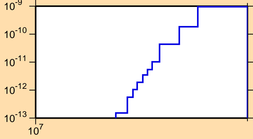
\sigma vs. E for ^{259}\text{Md}(n,3n\alpha)
