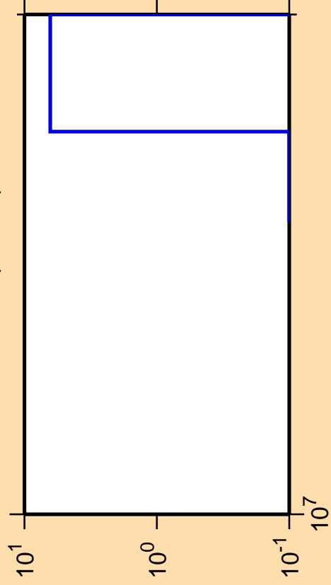
\Delta\sigma/\sigma vs. E for ^{259}\text{Md} (mt 42)
