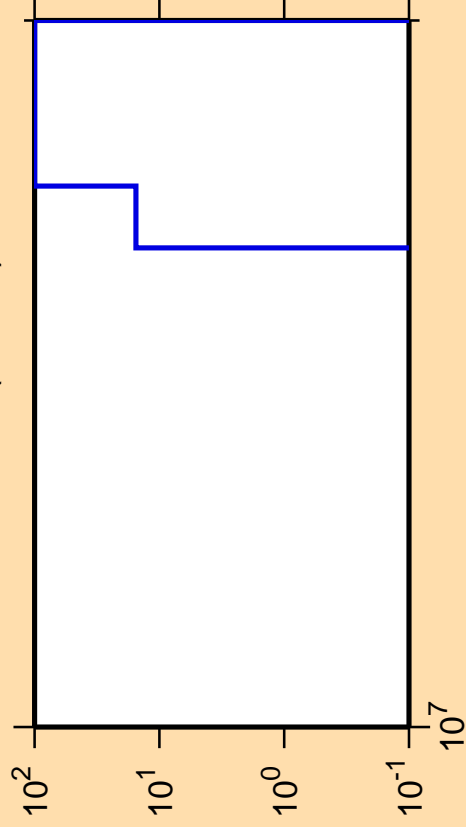
\Delta\sigma/\sigma vs. E for ^{259}\text{Md}(n,\text{He}3)
