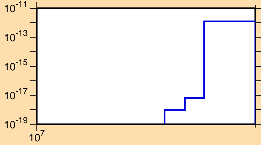
\sigma vs. E for ^{259}\text{Md} (mt 42)
