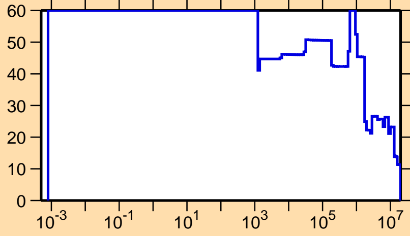
\Delta\sigma/\sigma vs. E for ^{259}\text{Md}(n,\text{el.})
