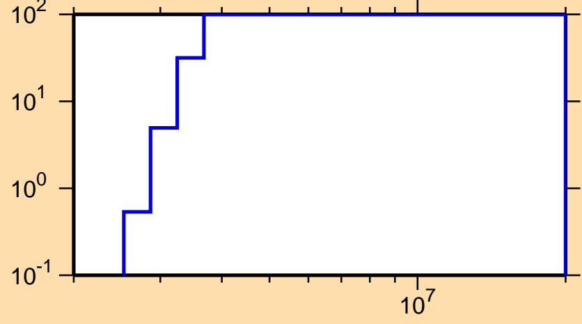
\Delta\sigma/\sigma vs. E for ^{259}\text{Md}(n,p)
