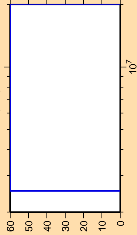
\Delta\sigma/\sigma vs. E for ^{259}\text{Md}(n,\alpha)
