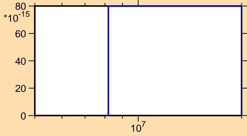
\sigma vs. E for ^{259}\text{Md}(\text{mt } 11)
