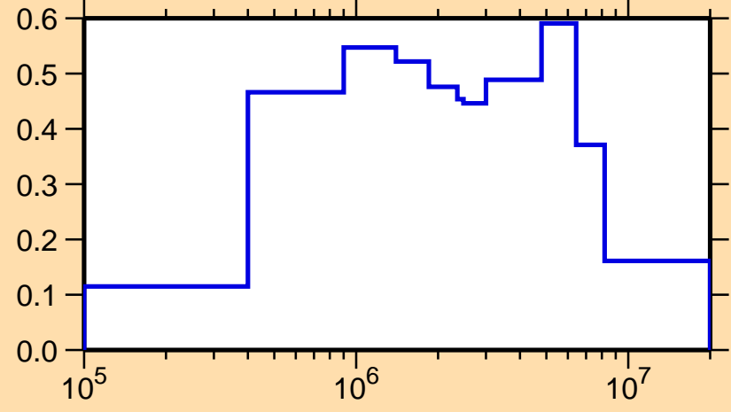
\sigma vs. E for ^{259}\text{Md}(n,n\text{cont.})
