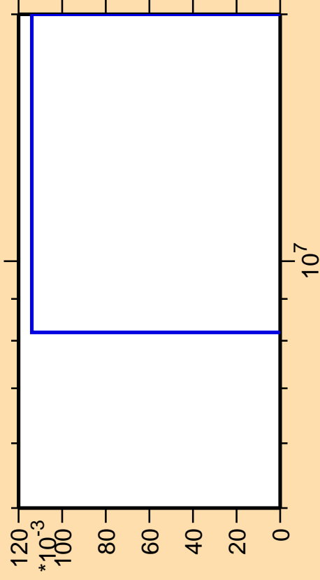
\Delta\sigma/\sigma vs. E for ^{259}\text{Md}(\text{mt } 11)
