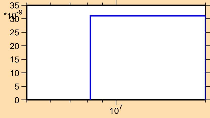
\sigma vs. E for ^{259}\text{Md}(n,2n\alpha)
