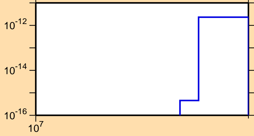
\sigma vs. E for ^{260}\text{Md} (mt 11)
