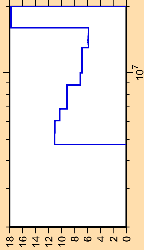
\Delta\sigma/\sigma vs. E for ^{260}\text{Md}(n,f)
