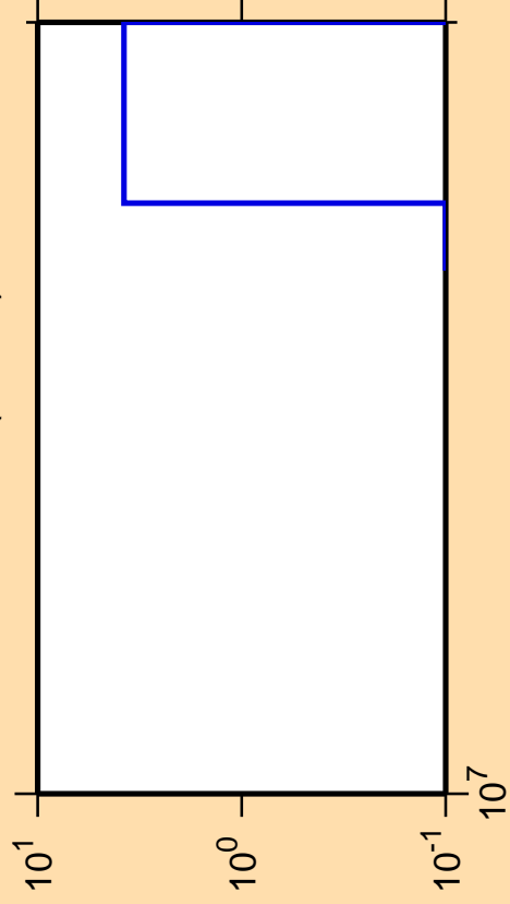
\Delta\sigma/\sigma vs. E for ^{260}\text{Md} (mt 11)
