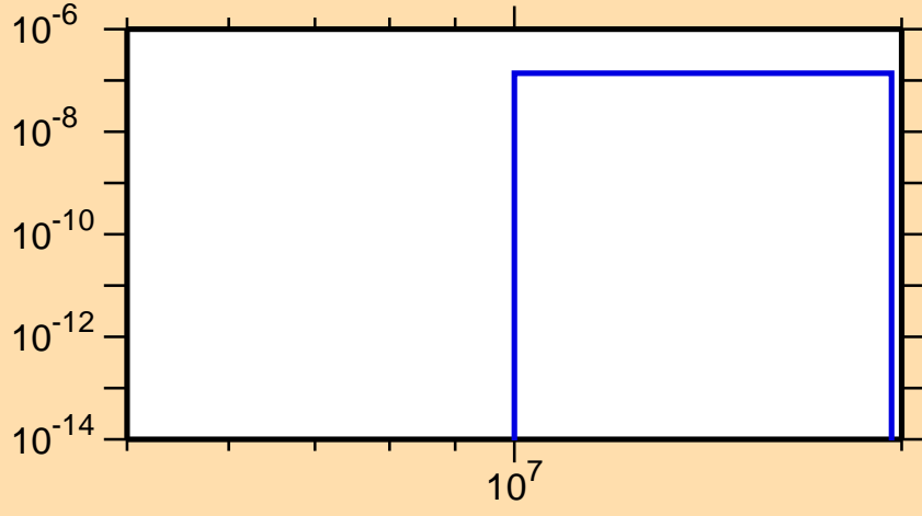
\sigma vs. E for ^{260}\text{Md}(n,\text{nd})
