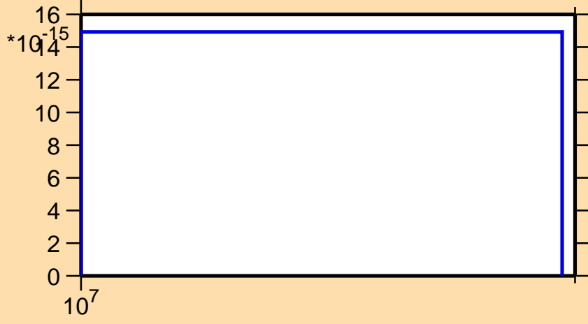
\sigma vs. E for ^{260}\text{Md} (mt 11)
