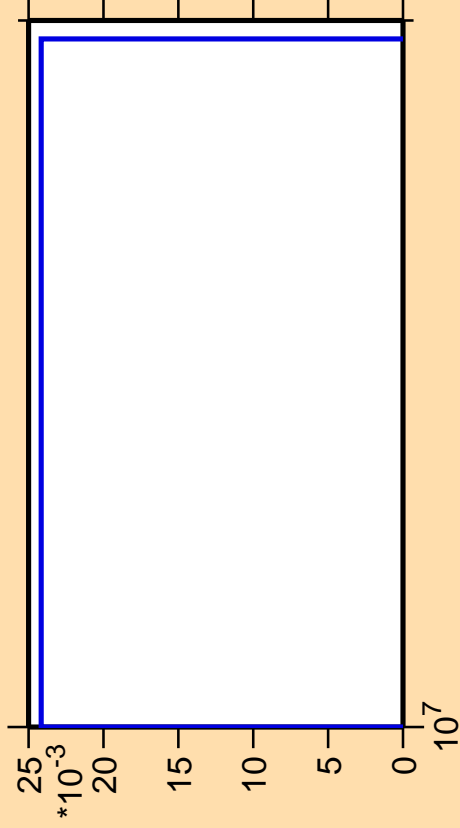
\Delta\sigma/\sigma vs. E for ^{260}\text{Md} (mt 11)
