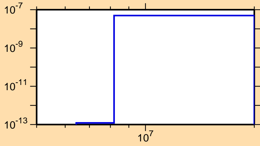
\sigma vs. E for ^{260}\text{Md}(n,2n\alpha)
