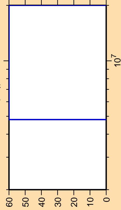
\Delta\sigma/\sigma vs. E for ^{260}\text{Md}(n,\gamma)
