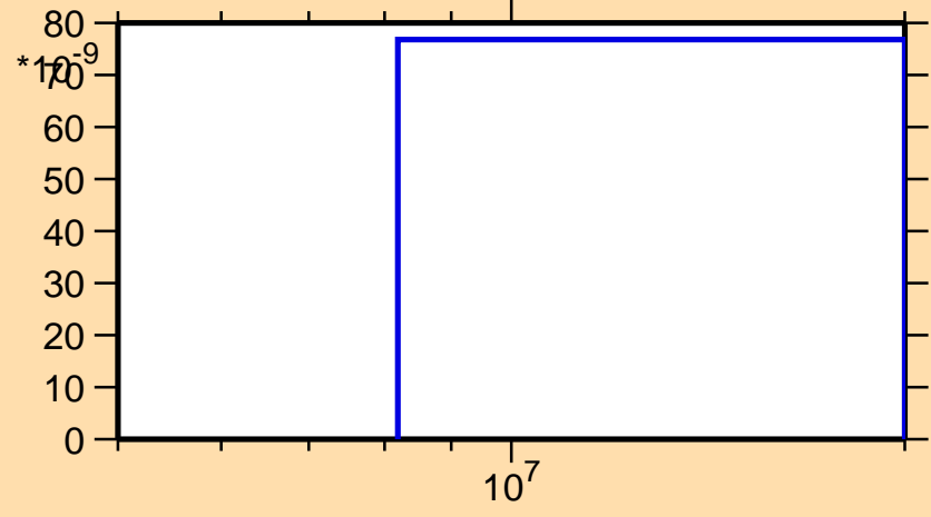
\sigma vs. E for ^{260}\text{Md}(n,nt)
