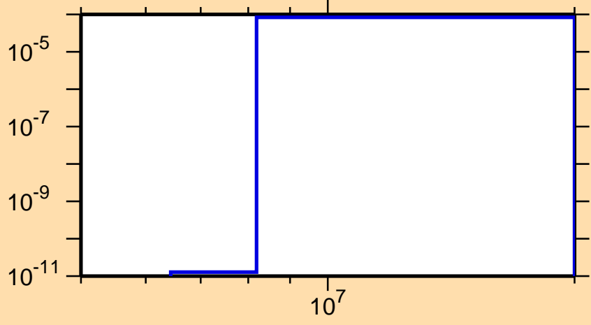
\sigma vs. E for ^{260}\text{Md}(n,t)
