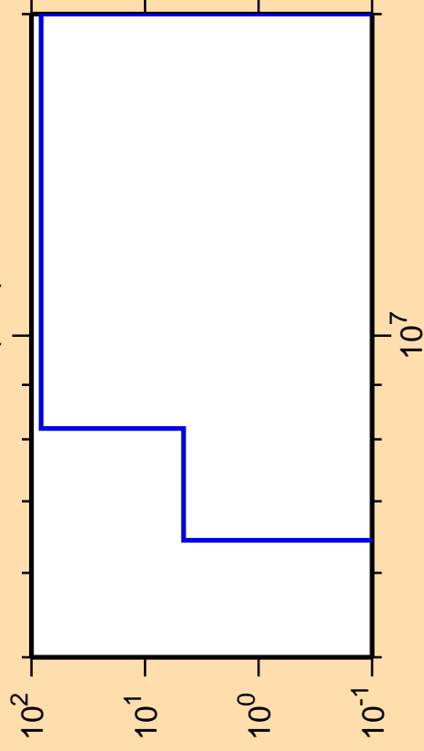
\Delta\sigma/\sigma vs. E for ^{260}\text{Md}(n,d)
