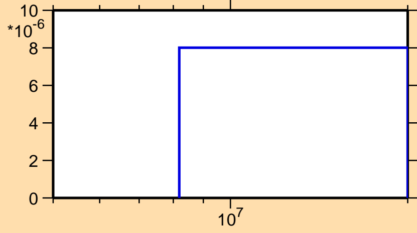
\sigma vs. E for ^{260}\text{Md}(n,np)
