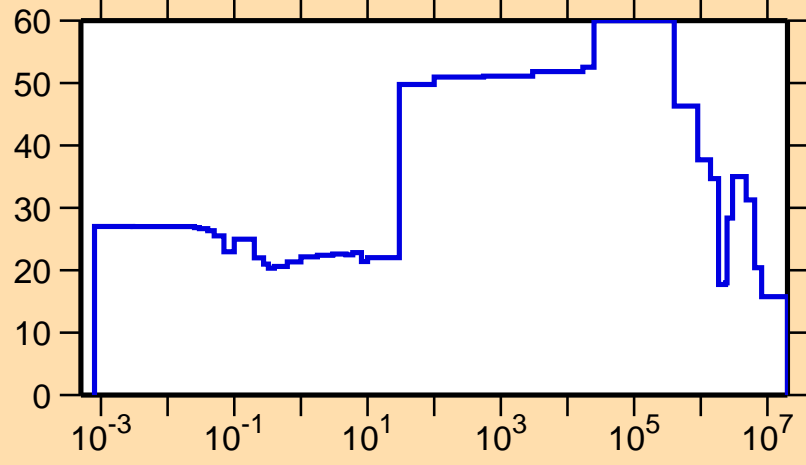
\Delta\sigma/\sigma vs. E for ^{260}\text{Md}(n,\text{el.})
