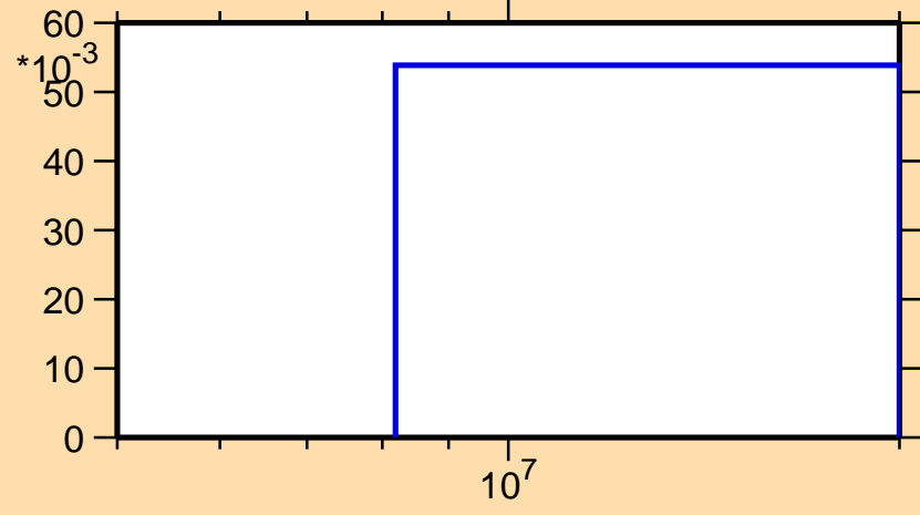
\sigma vs. E for ^{260}\text{Md}(n,3n)
