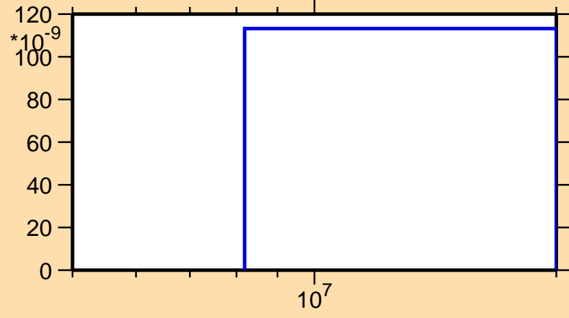
\sigma vs. E for ^{260}\text{Md}(n,\text{nd})
