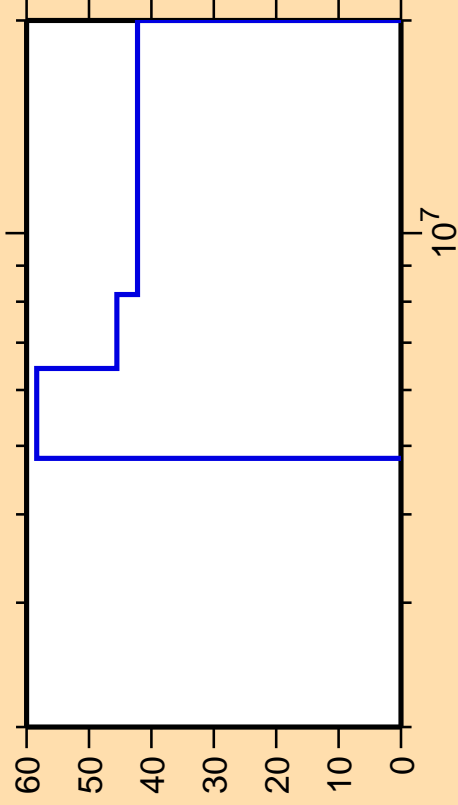
\Delta\sigma/\sigma vs. E for ^{260}\text{Md}(n, n_{\text{cont}}) .
