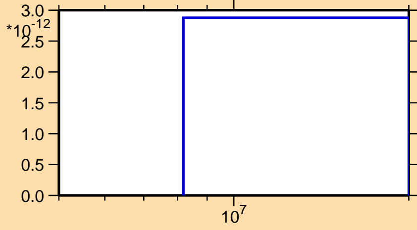
\sigma vs. E for ^{260}\text{Md}(n,3n\alpha)
