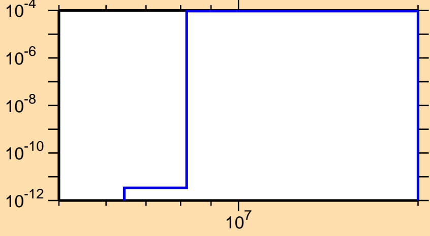
\sigma vs. E for ^{260}\text{Md}(n,d)
