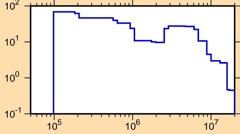
\Delta\sigma/\sigma vs. E for ^{262}\text{Md}(n,f)
