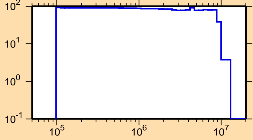
\Delta\sigma/\sigma vs. E for ^{262}\text{Md}(n,n_1)
