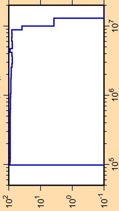
\Delta\sigma/\sigma vs. E for ^{262}\text{Md}(n,n_1)
