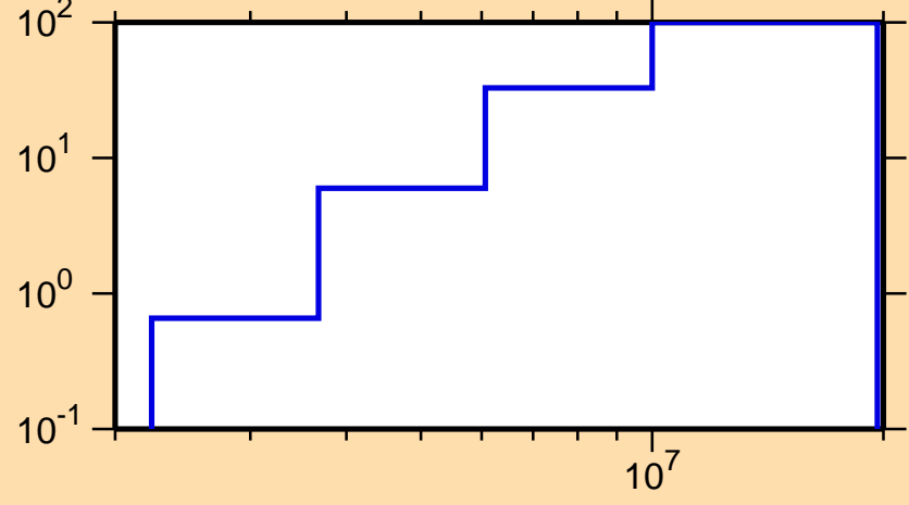
\Delta\sigma/\sigma vs. E for ^{262}\text{Md}(n,p)
