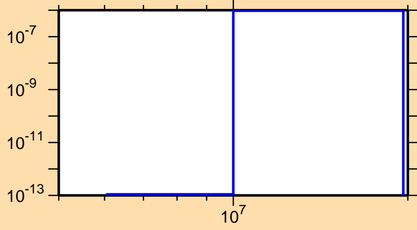
\sigma vs. E for ^{262}\text{Md}(n,np)
