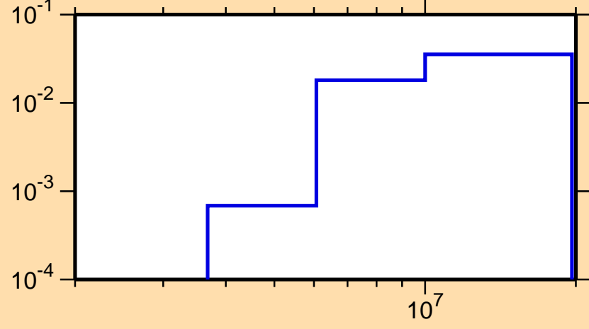
\sigma vs. E for ^{262}\text{Md}(n,2n)
