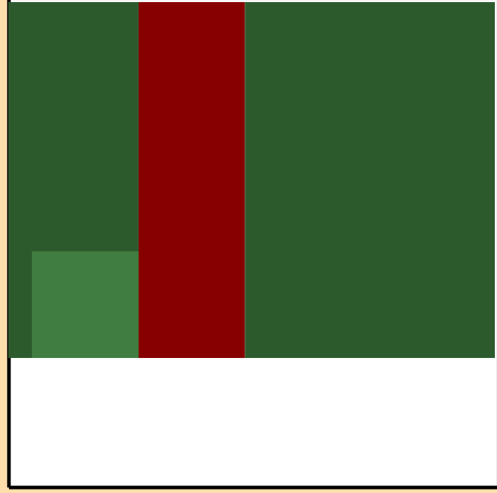
\Delta\sigma/\sigma vs. E for ^{262}\text{Md}(n,\text{nonel.})
