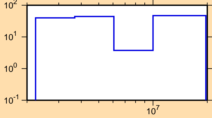
\Delta\sigma/\sigma vs. E for ^{262}\text{Md}(n,\gamma)
