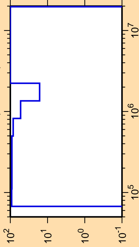
\Delta\sigma/\sigma vs. E for ^{262}\text{Md}(n,\text{ncont.})
