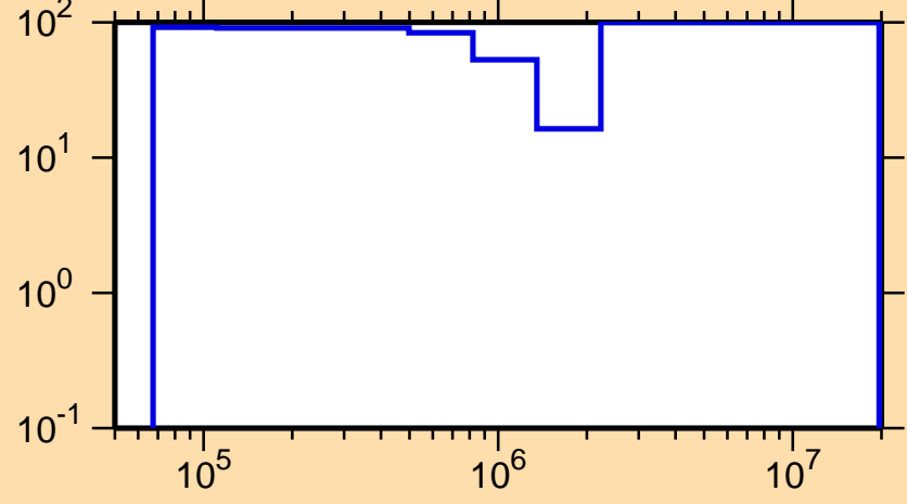
\Delta\sigma/\sigma vs. E for ^{262}\text{Md}(n,n\text{cont.})
