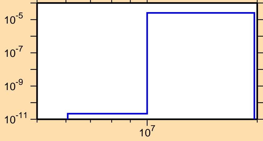
\sigma vs. E for ^{262}\text{Md}(n,d)
