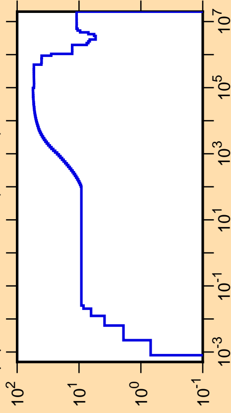
\Delta\mu/\mu vs. E for ^{126}\text{Nd}(\text{mt251})
