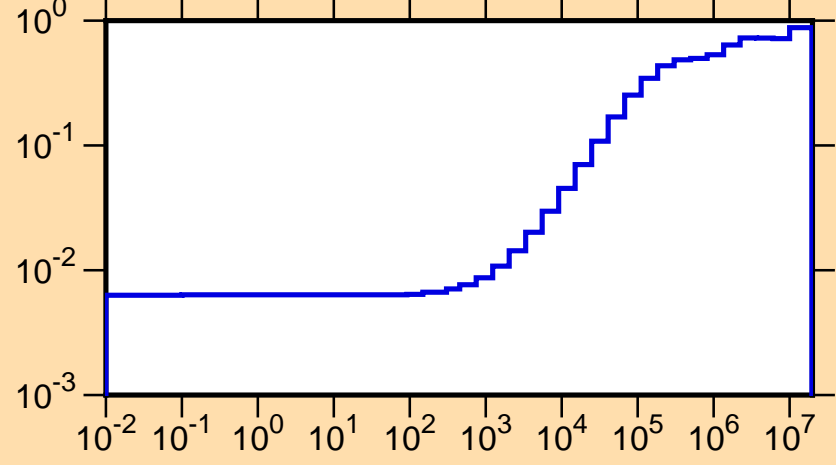
\mu vs. E for ^{126}\text{Nd}(\text{mt251})
