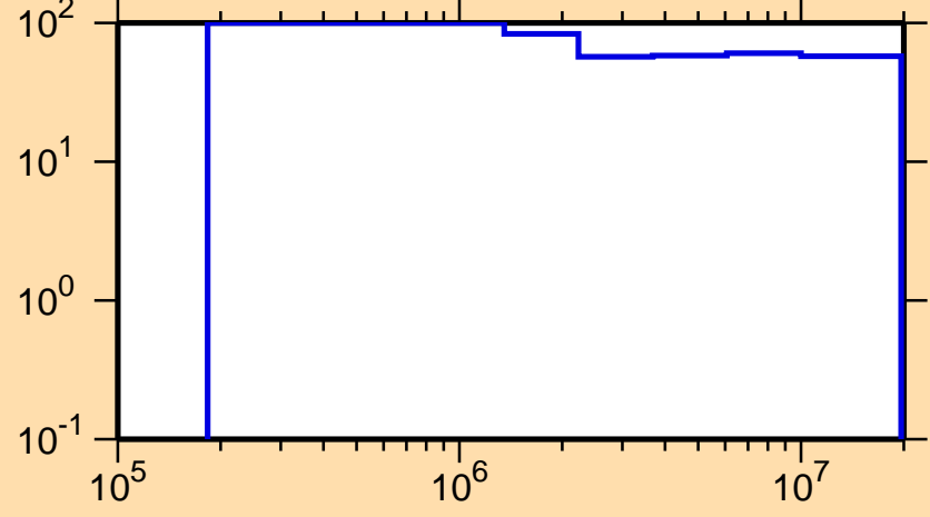
\Delta\sigma/\sigma vs. E for ^{126}\text{Nd}(n,n_1)
