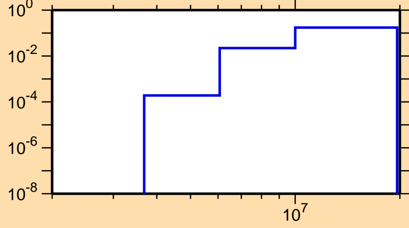
\sigma vs. E for ^{126}\text{Nd}(n,np)
