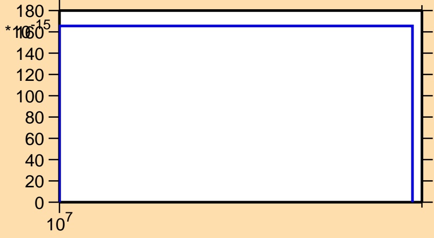
\sigma vs. E for ^{126}\text{Nd}(n,2n\alpha)
