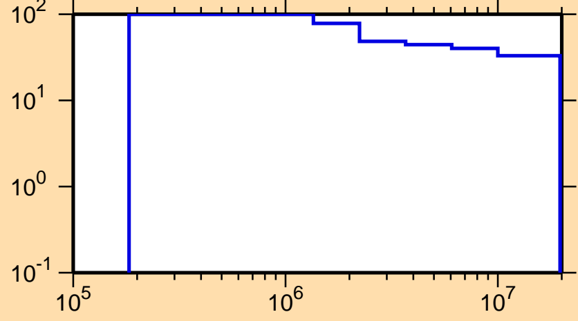
\Delta\sigma/\sigma vs. E for ^{126}\text{Nd}(n,\text{inel.})
