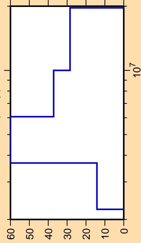
\Delta\sigma/\sigma vs. E for ^{126}\text{Nd}(n,np)
