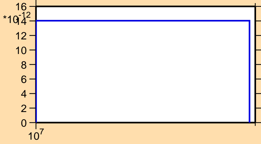
\sigma vs. E for ^{126}\text{Nd} (mt 34)
