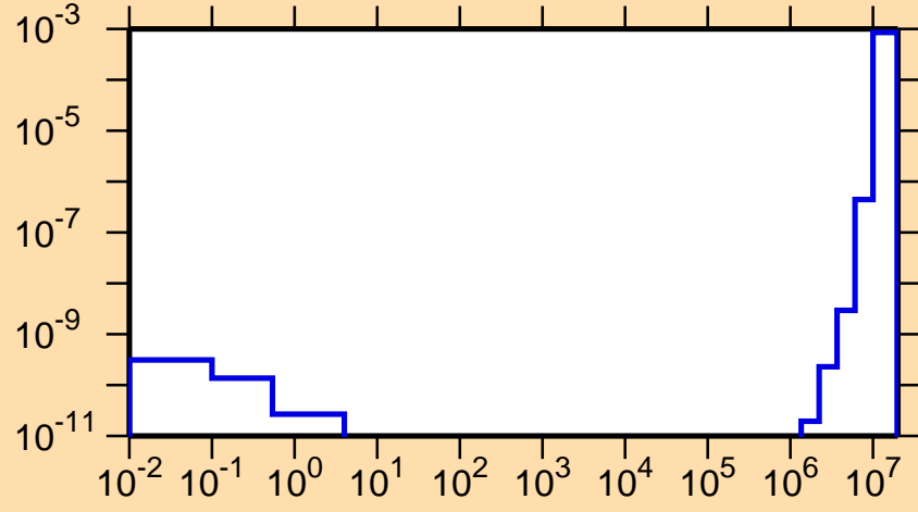
\sigma vs. E for ^{126}\text{Nd}(n,\text{He3})
