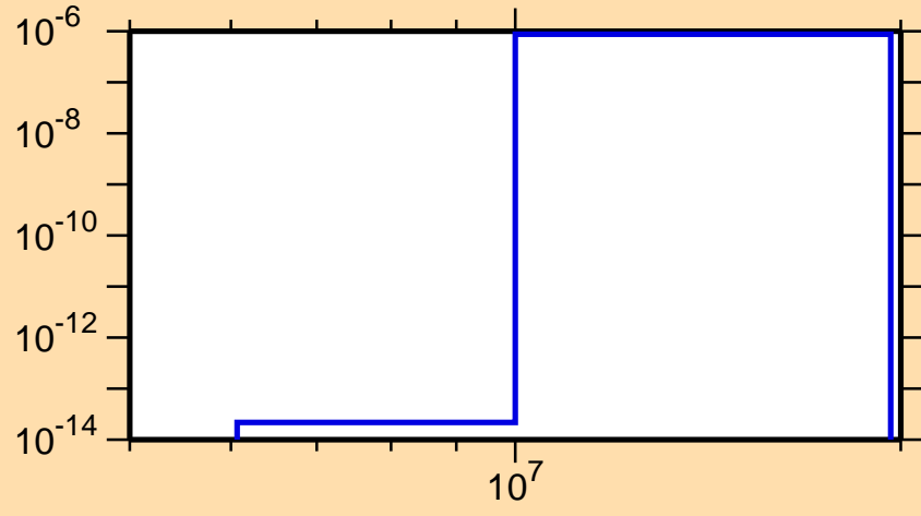
\sigma vs. E for ^{126}\text{Nd}(\text{mt } 45)
