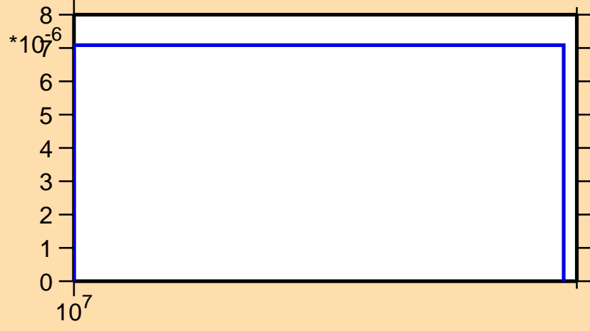
\sigma vs. E for ^{126}\text{Nd}(n,2n)
