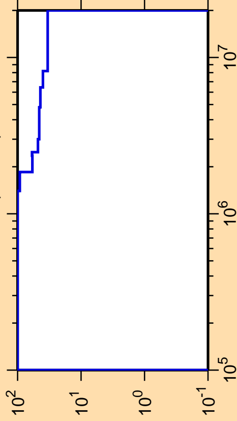
\Delta\sigma/\sigma vs. E for ^{126}\text{Nd}(n,\text{inel.})
