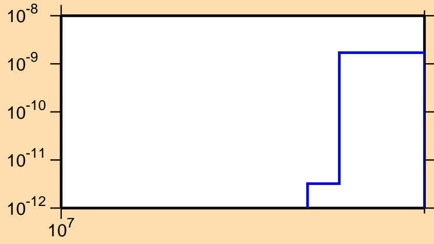
\sigma vs. E for ^{130}\text{Nd}(n,2n\alpha)
