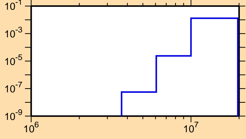
\sigma vs. E for ^{130}\text{Nd}(n,p\alpha)
