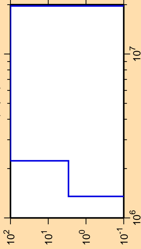
\Delta\sigma/\sigma vs. E for ^{130}\text{Nd}(n,p\alpha)
