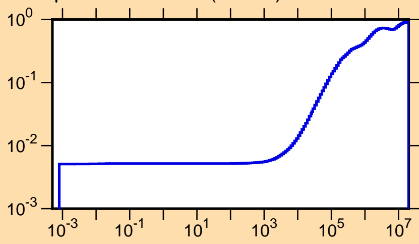
\mu vs. E for ^{132}\text{Nd}(\text{mt251})
