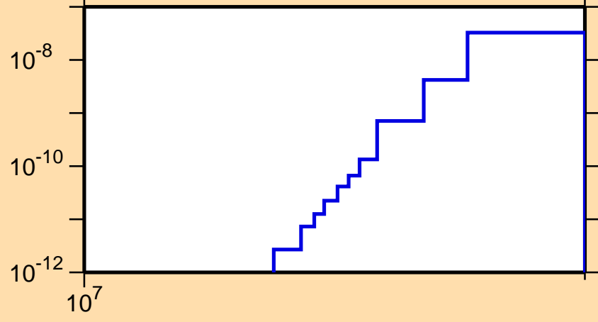
\sigma vs. E for ^{132}\text{Nd}(\text{mt117})
