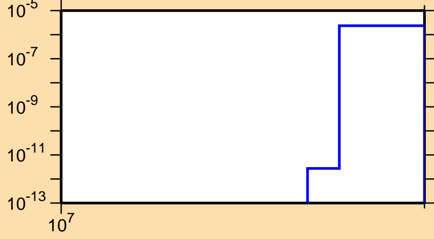
\sigma vs. E for ^{132}\text{Nd}(n,2np)
