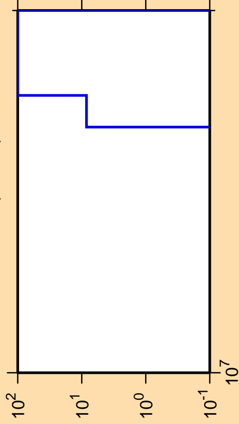
\Delta\sigma/\sigma vs. E for ^{132}\text{Nd} (mt 34)
