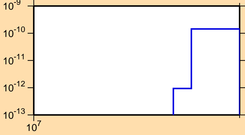
\sigma vs. E for ^{132}\text{Nd} (mt 34)
