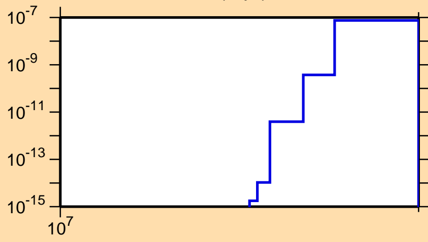
\sigma vs. E for ^{132}\text{Nd}(n,\text{pt})
