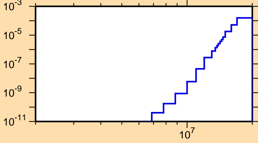
\sigma vs. E for ^{132}\text{Nd}(n,\text{He}3)
