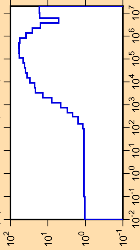
\Delta\mu/\mu vs. E for ^{132}\text{Nd}(\text{mt251})
