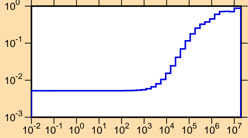
\mu vs. E for ^{132}\text{Nd}(\text{mt251})
