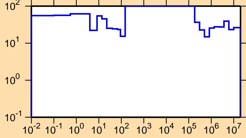
\Delta\sigma/\sigma vs. E for ^{132}\text{Nd}(n,\text{el.})
