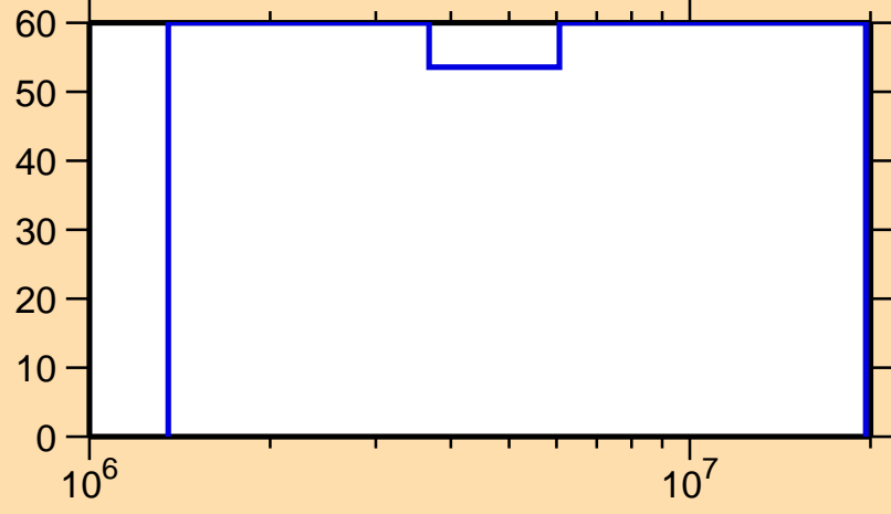
\Delta\sigma/\sigma vs. E for ^{132}\text{Nd}(n,n\text{cont.})
