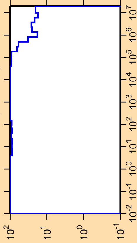
\Delta\sigma/\sigma vs. E for ^{132}\text{Nd}(n,\text{nonel.})
