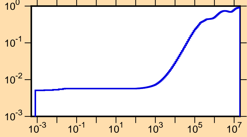
\mu vs. E for ^{133}\text{Nd}(\text{mt251})
