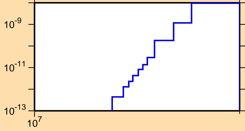
\sigma vs. E for ^{133}\text{Nd}(\text{mt117})
