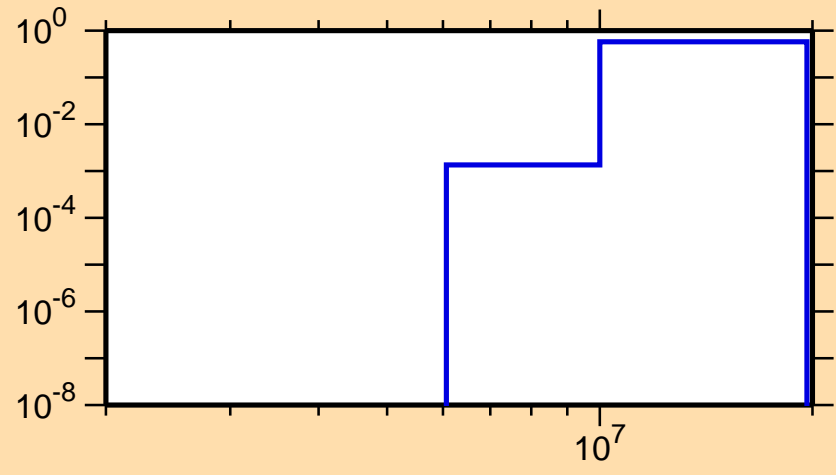
\sigma vs. E for ^{133}\text{Nd}(n,np)
