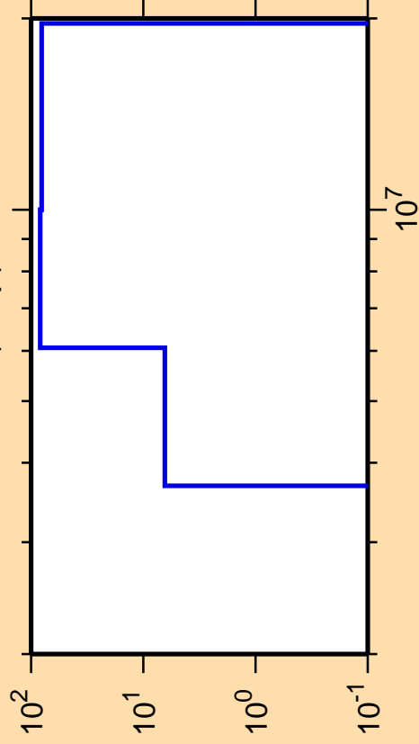
\Delta\sigma/\sigma vs. E for ^{133}\text{Nd}(n,np)
