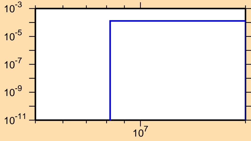
\sigma vs. E for ^{133}\text{Nd}(n,t)
