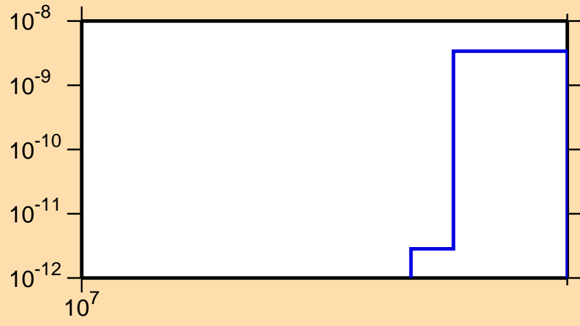
\sigma vs. E for ^{134}\text{Nd}(n,\text{pt})
