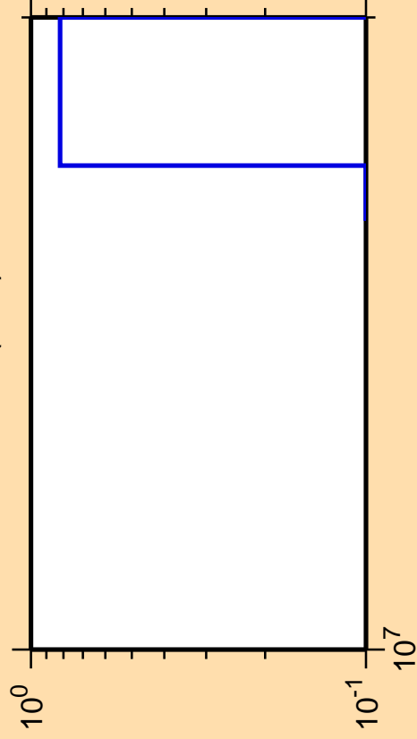
\Delta\sigma/\sigma vs. E for ^{134}\text{Nd}(n,nt)
