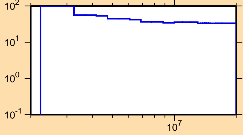
\Delta\sigma/\sigma vs. E for ^{134}\text{Nd}(n,ncont.)
