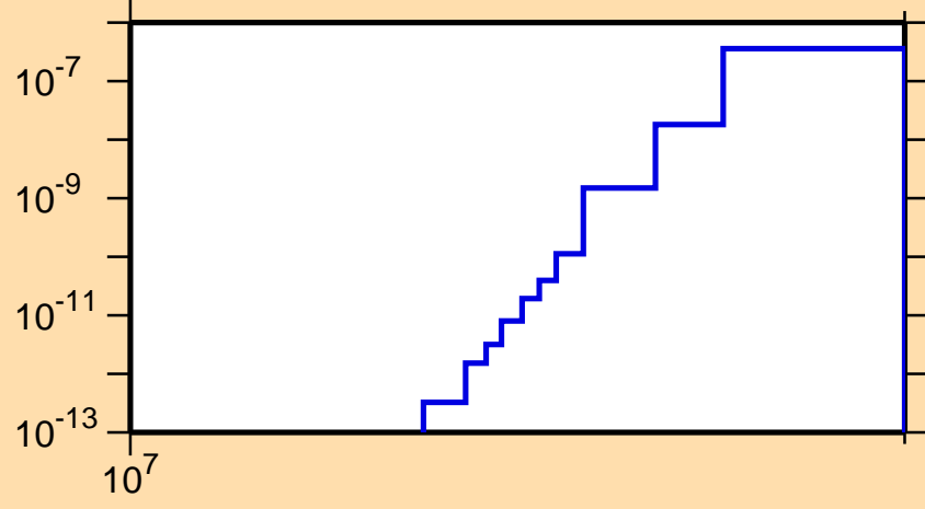
\sigma vs. E for ^{134}\text{Nd}(\text{mt } 45)
