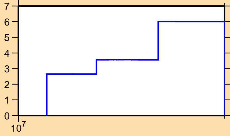
\Delta\sigma/\sigma vs. E for ^{134}\text{Nd}(n,\text{tot.})
