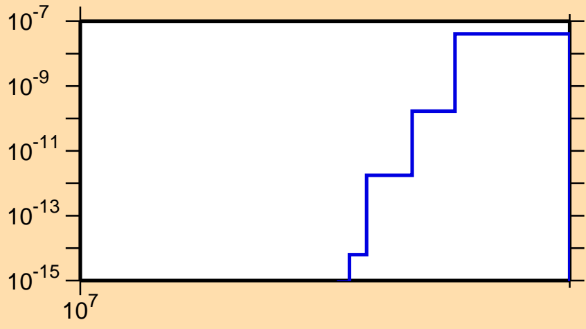
\sigma vs. E for ^{134}\text{Nd}(n,2n\alpha)
