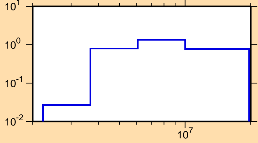
\sigma vs. E for ^{134}\text{Nd}(n,n\text{cont.})
