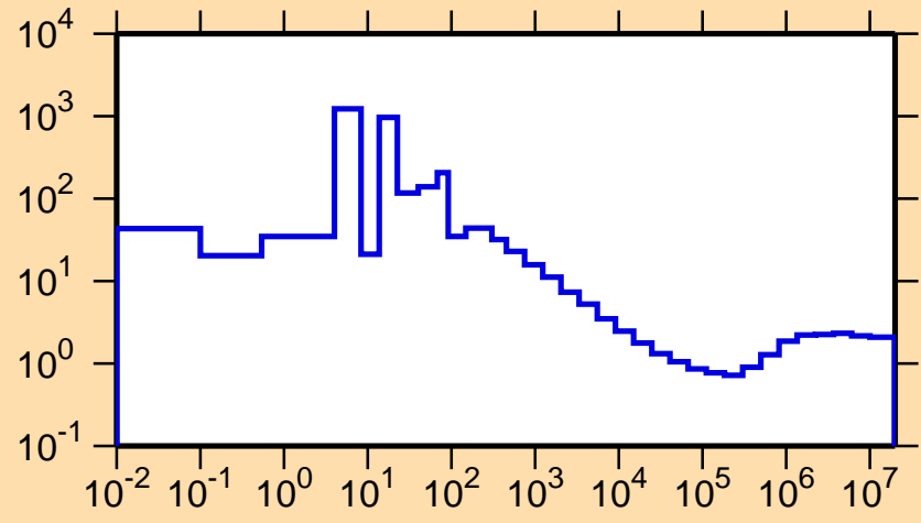
\sigma vs. E for ^{134}\text{Nd}(n,\text{nonel.})
