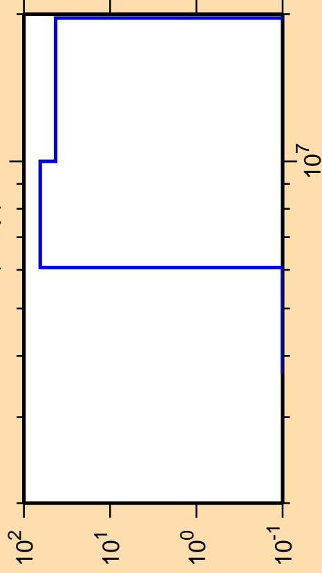
\Delta\sigma/\sigma vs. E for ^{134}\text{Nd}(n,np)
