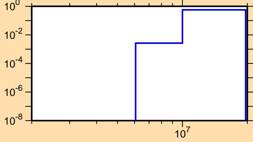
\sigma vs. E for ^{134}\text{Nd}(n,np)
