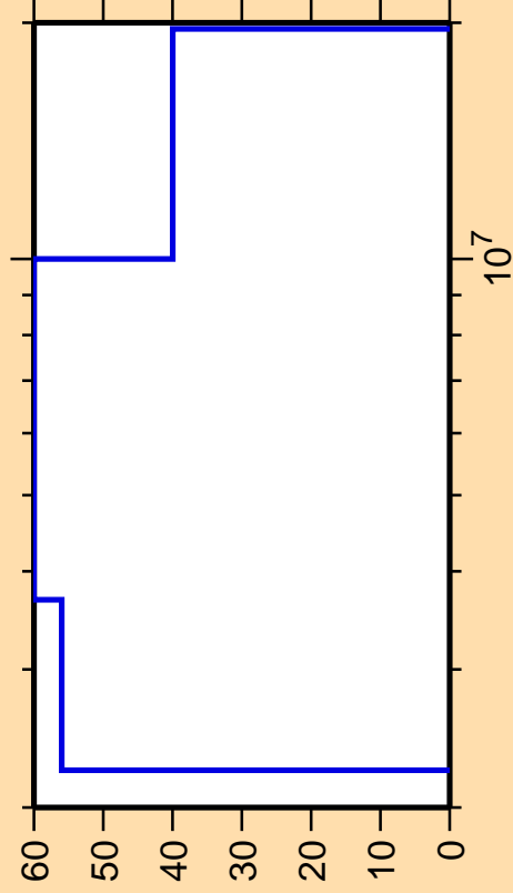
\Delta\sigma/\sigma vs. E for ^{134}\text{Nd}(n,\gamma)
