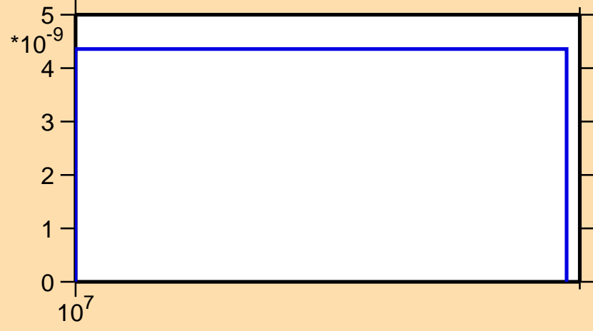
\sigma vs. E for ^{134}\text{Nd} (mt 45)
