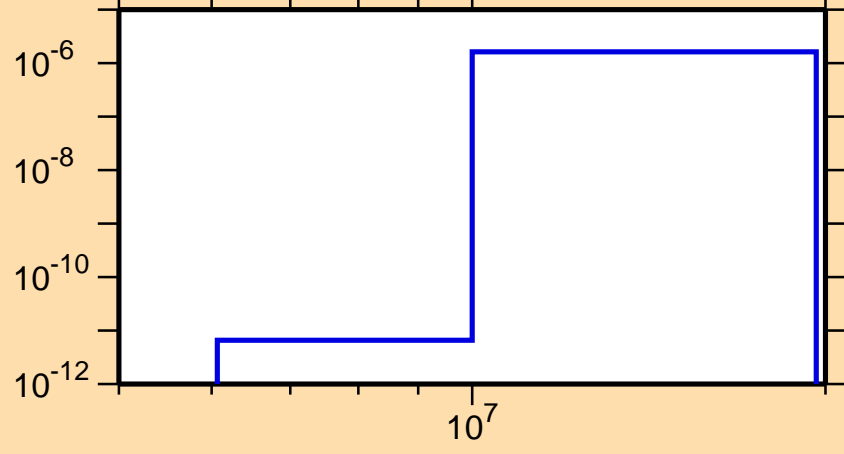
\sigma vs. E for ^{134}\text{Nd}(n,\text{He3})
