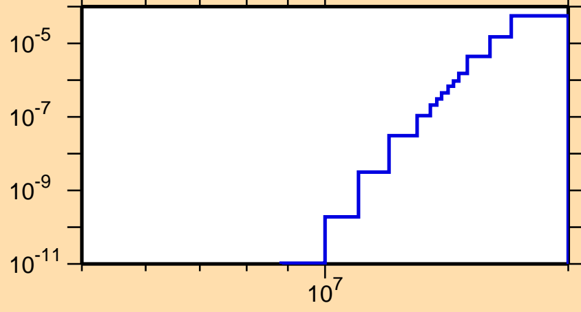
\sigma vs. E for ^{135}\text{Nd}(n,\text{He3})
