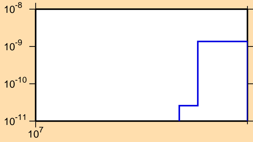
\sigma vs. E for ^{135}\text{Nd}(\text{mt } 34)
