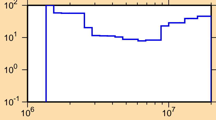
\Delta\sigma/\sigma vs. E for ^{135}\text{Nd}(n,n\text{cont.})
