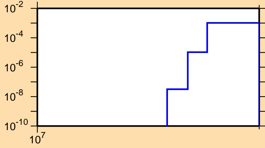
\sigma vs. E for ^{135}\text{Nd}(n,2np)
