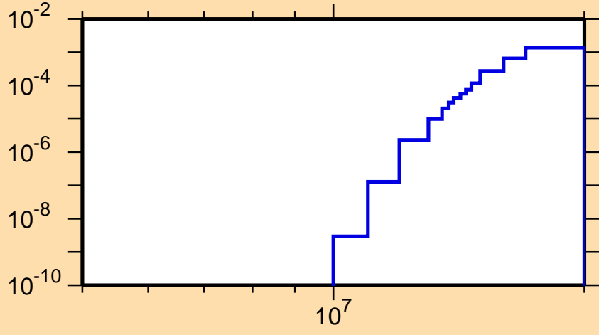
\sigma vs. E for ^{135}\text{Nd}(n,t)
