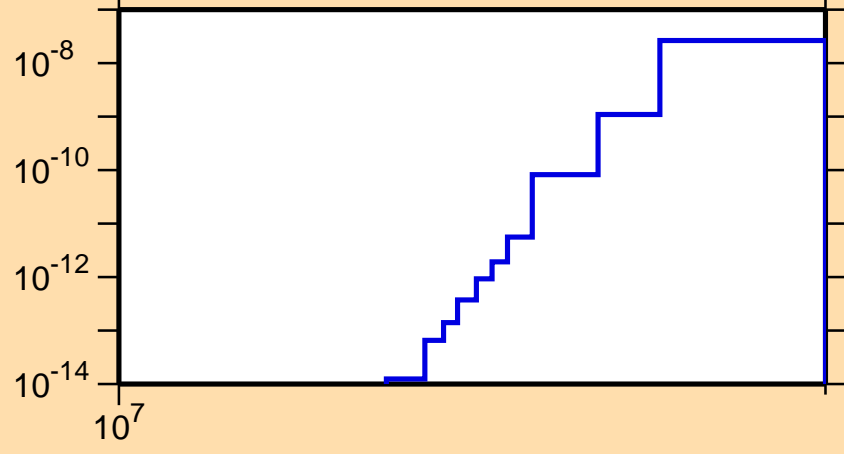
\sigma vs. E for ^{135}\text{Nd}(\text{mt } 45)
