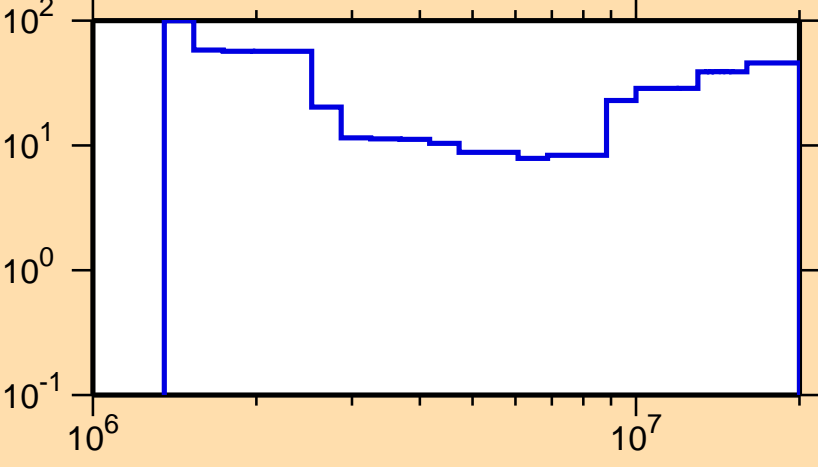
\Delta\sigma/\sigma vs. E for ^{135}\text{Nd}(n,n\text{cont.})
