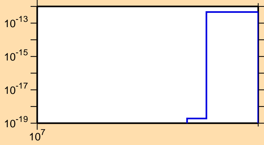
\sigma vs. E for ^{135}\text{Nd}(n,\text{nt})
