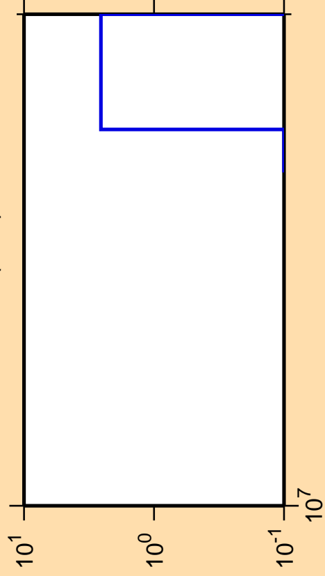
\Delta\sigma/\sigma vs. E for ^{135}\text{Nd}(n,\text{nt})
