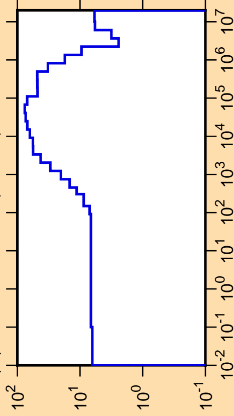
\Delta\mu/\mu vs. E for ^{135}\text{Nd}(\text{mt251})
