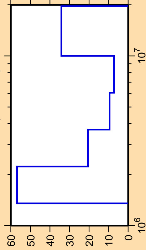
\Delta\sigma/\sigma vs. E for ^{135}\text{Nd}(n,\text{ncont.})
