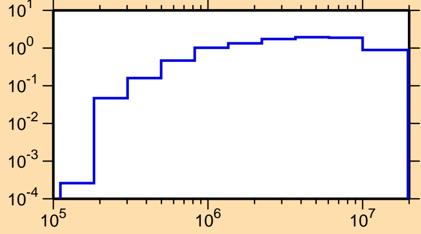
\sigma vs. E for ^{135}\text{Nd}(n,\text{inel.})
