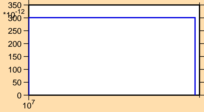
\sigma vs. E for ^{135}\text{Nd}(\text{mt } 45)
