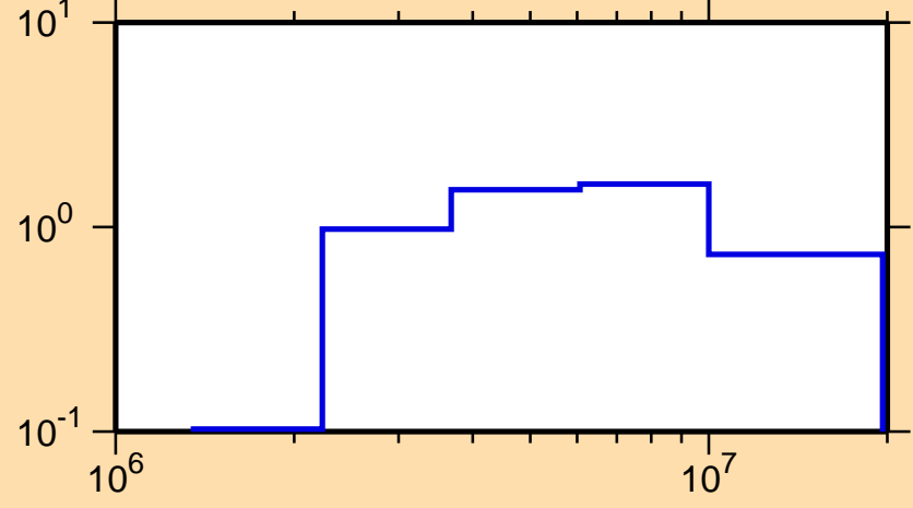
\sigma vs. E for ^{135}\text{Nd}(n,n\text{cont.})
