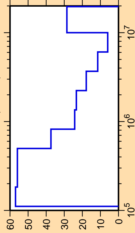
\Delta\sigma/\sigma vs. E for ^{135}\text{Nd}(n,\text{inel.})
