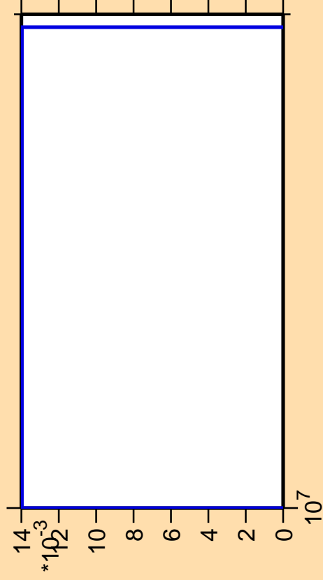
\Delta\sigma/\sigma vs. E for ^{135}\text{Nd}(n,\text{nt})
