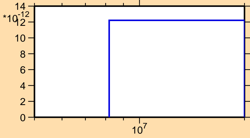
\sigma vs. E for ^{135}\text{Nd}(\text{mt } 34)
