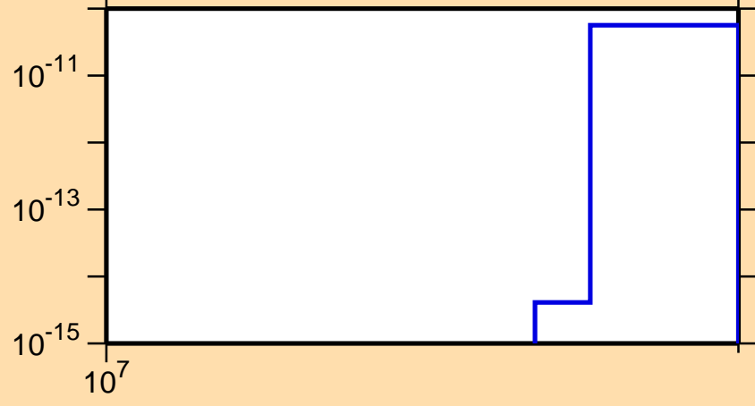
\sigma vs. E for ^{136}\text{Nd}(n,\text{pt})
