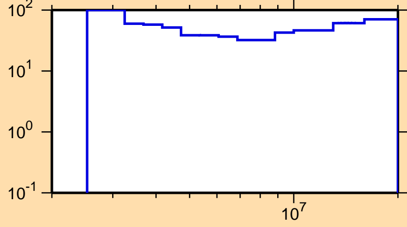
\Delta\sigma/\sigma vs. E for ^{136}\text{Nd}(n,n\text{cont.})
