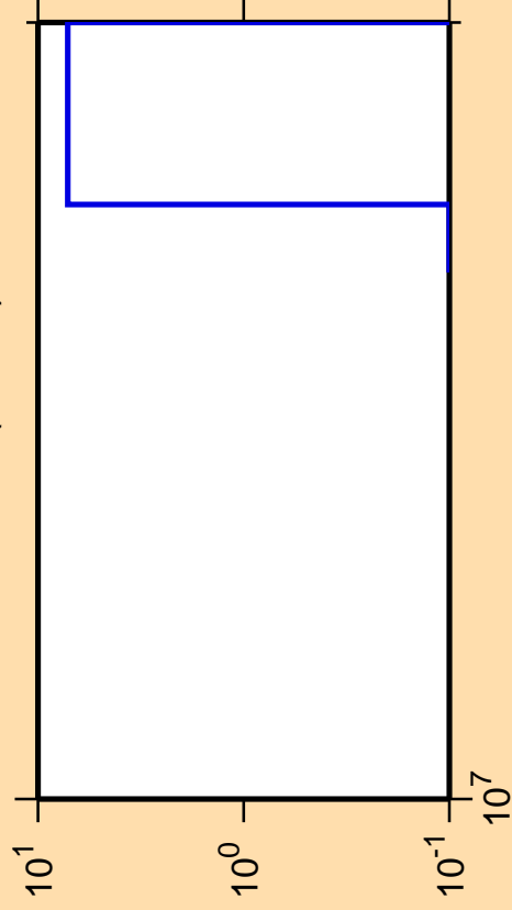
\Delta\sigma/\sigma vs. E for ^{136}\text{Nd}(\text{mt } 34)
