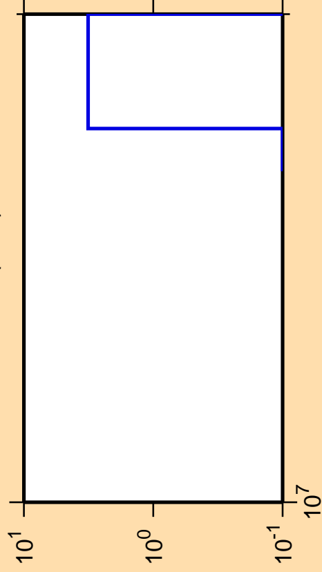
\Delta\sigma/\sigma vs. E for ^{136}\text{Nd}(n,\text{nt})
