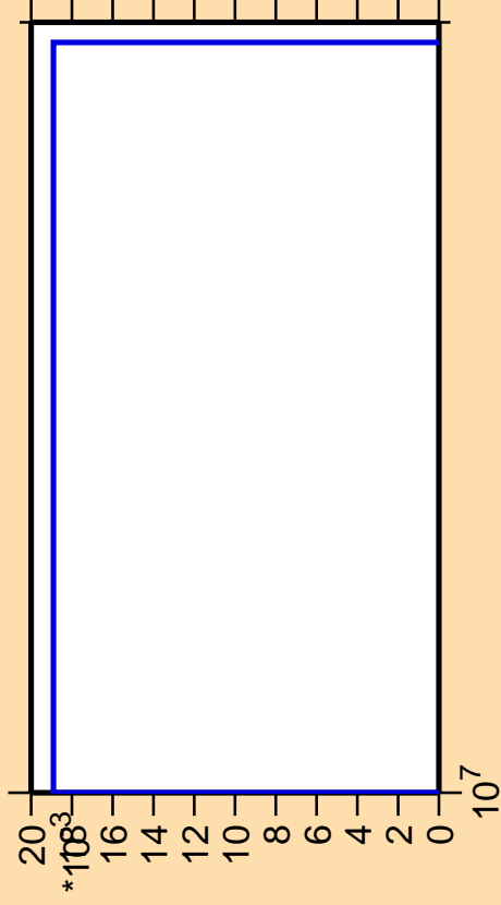
\Delta\sigma/\sigma vs. E for ^{136}\text{Nd}(n,\text{nt})
