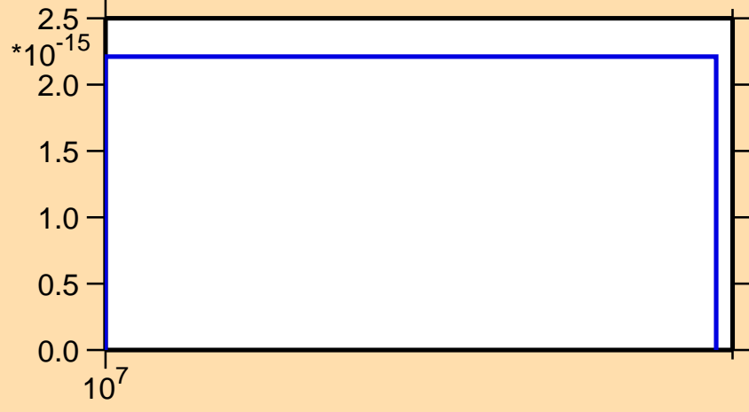
\sigma vs. E for ^{136}\text{Nd}(n,\text{nt})
