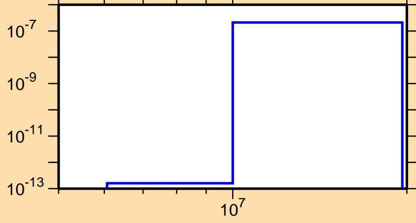
\sigma vs. E for ^{136}\text{Nd}(n,\text{He3})
