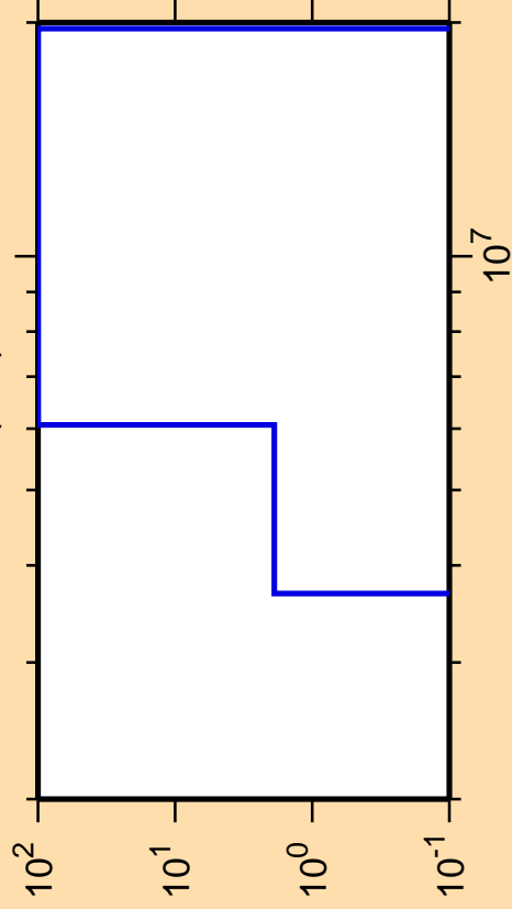
\Delta\sigma/\sigma vs. E for ^{136}\text{Nd}(n,d)
