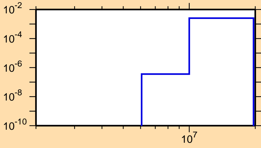
\sigma vs. E for ^{136}\text{Nd}(n,d)
