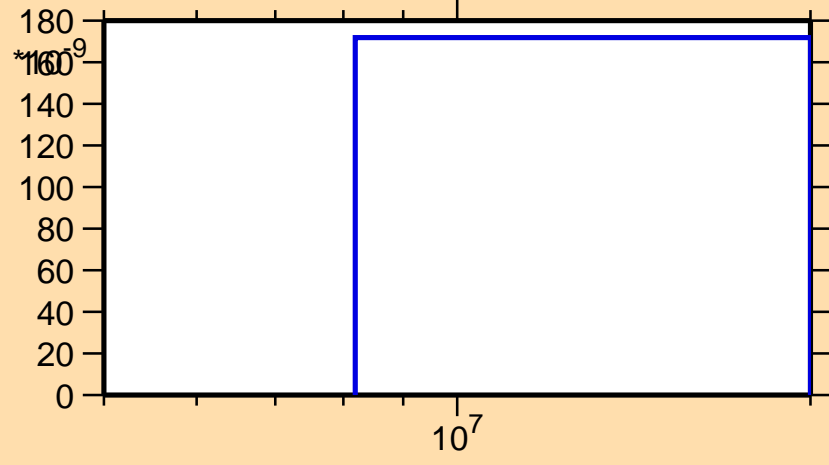
\sigma vs. E for ^{136}\text{Nd}(n,\text{He3})
