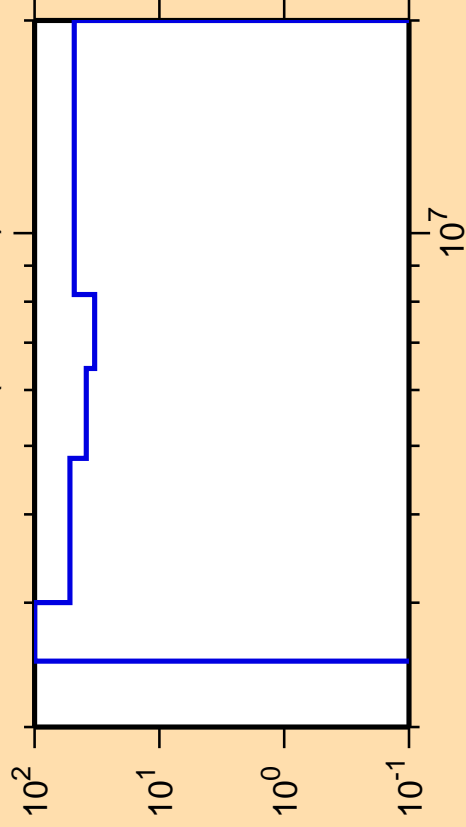
\Delta\sigma/\sigma vs. E for ^{136}\text{Nd}(n,\text{ncont.})
