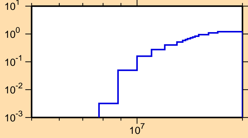
\sigma vs. E for ^{137}\text{Nd}(n,2n)
