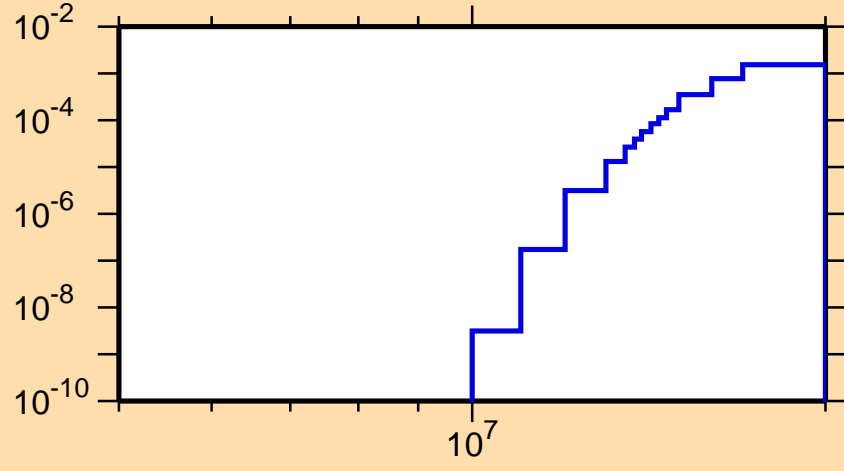
\sigma vs. E for ^{137}\text{Nd}(n,t)
