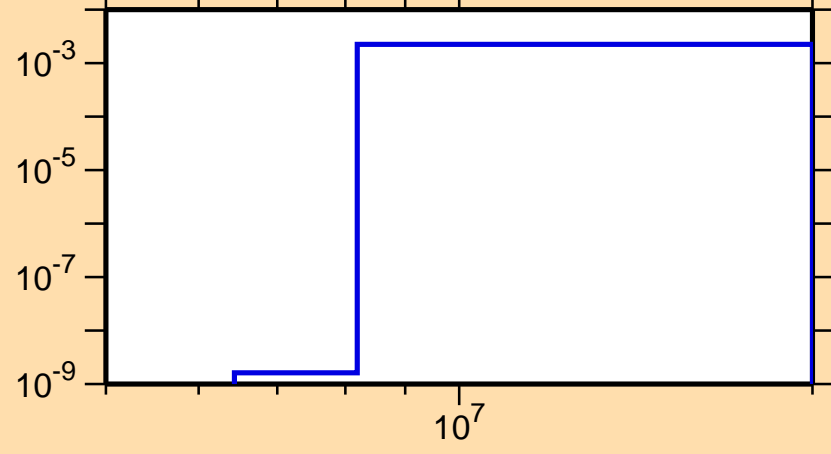
\sigma vs. E for ^{139}\text{Nd}(n,d)
