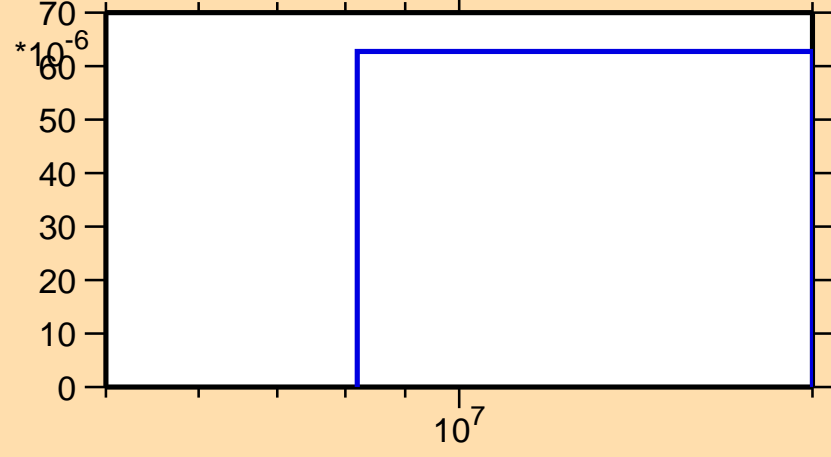
\sigma vs. E for ^{139}\text{Nd}(n,t)
