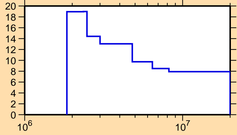
\Delta\sigma/\sigma vs. E for ^{139}\text{Nd}(n,n\text{onel.})
