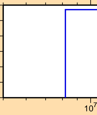
\sigma vs. E for ^{139}\text{Nd}(n,\text{nt})
