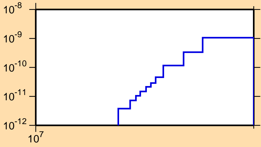
\sigma vs. E for ^{144}\text{Nd}(n,p\alpha)
