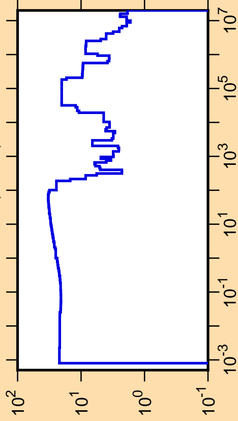
\Delta\sigma/\sigma vs. E for ^{144}\text{Nd}(n,\text{tot.})
