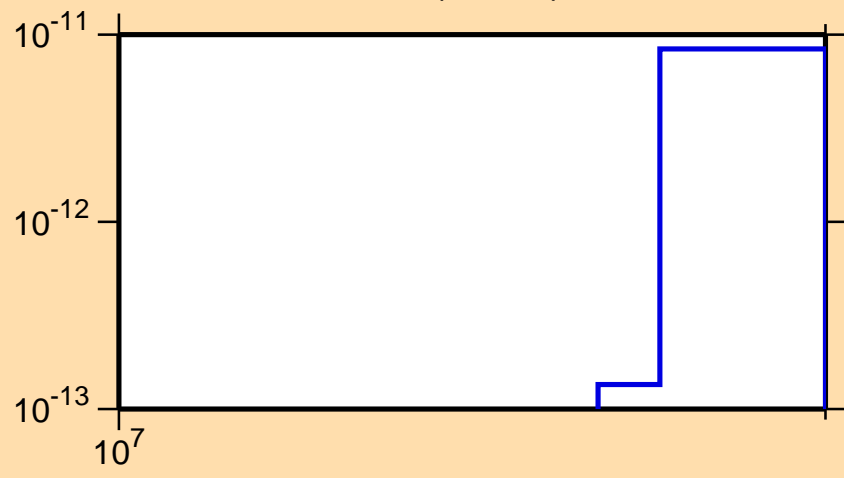
\sigma vs. E for ^{144}\text{Nd}(\text{mt } 45)
