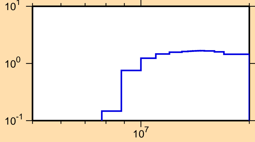
\sigma vs. E for ^{144}\text{Nd}(n,2n)
