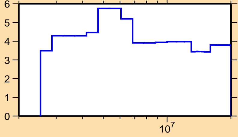
\Delta\sigma/\sigma vs. E for ^{144}\text{Nd}(n,n\text{onel.})
