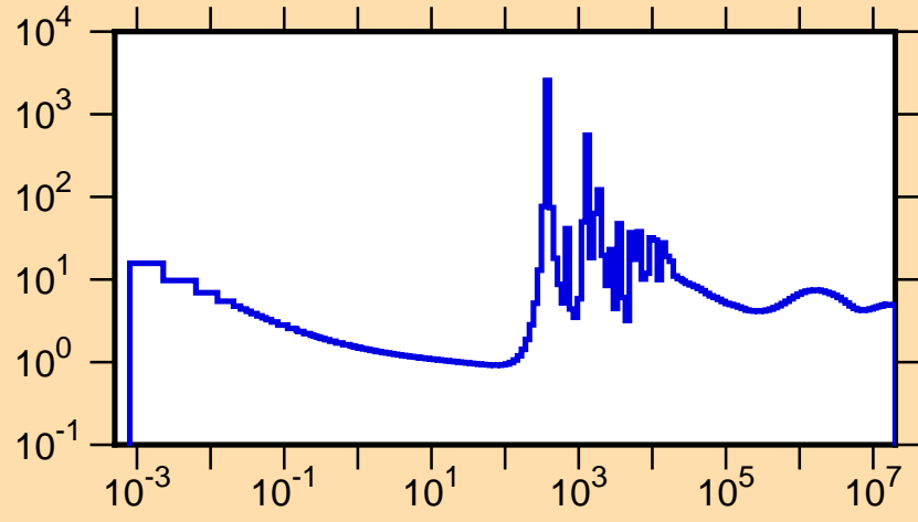
\sigma vs. E for ^{144}\text{Nd}(n,\text{tot.})
