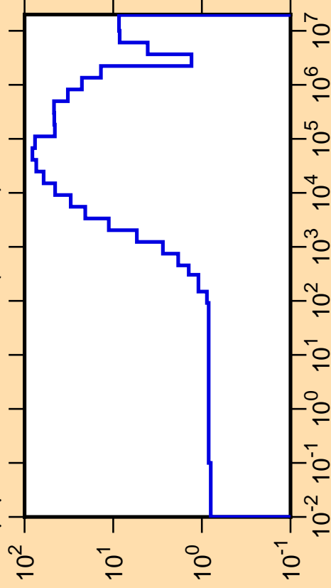
\Delta\mu/\mu vs. E for ^{144}\text{Nd}(\text{mt251})
