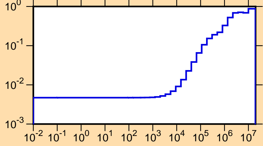
\mu vs. E for ^{144}\text{Nd}(\text{mt251})
