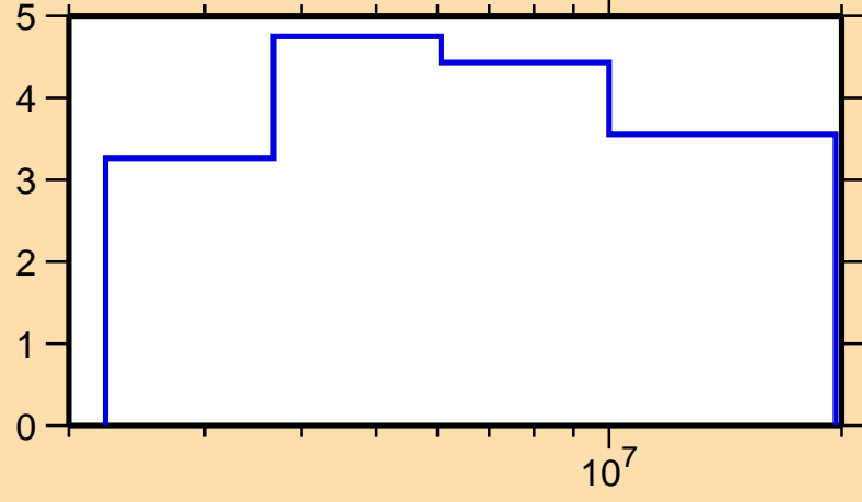
\Delta\sigma/\sigma vs. E for ^{144}\text{Nd}(n,\text{nonel.})
