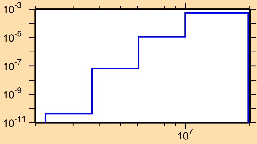
\sigma vs. E for ^{144}\text{Nd}(n,n\alpha)
