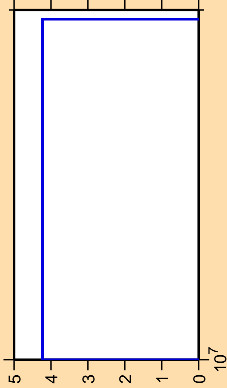
\Delta\sigma/\sigma vs. E for ^{144}\text{Nd}(\text{mt117})
