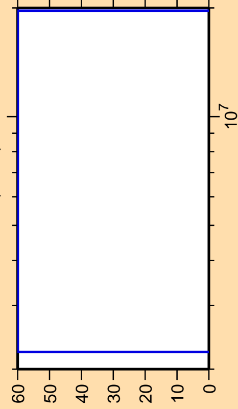
\Delta\sigma/\sigma vs. E for ^{144}\text{Nd}(n,n\alpha)
