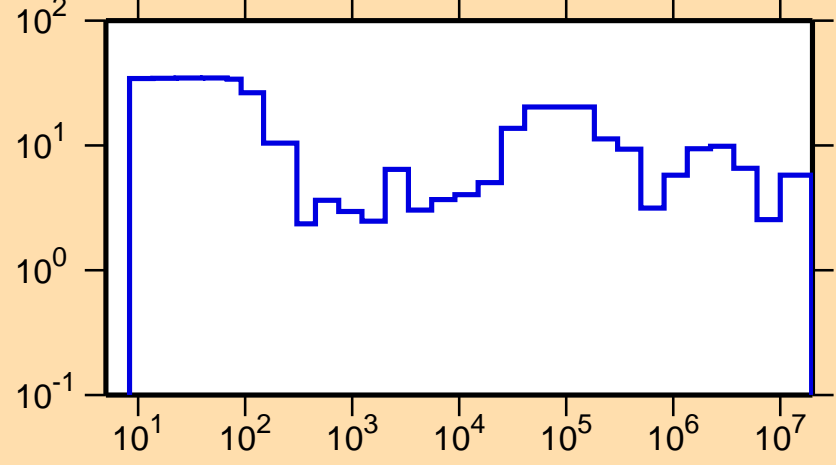
\Delta\sigma/\sigma vs. E for ^{144}\text{Nd}(n,\text{el.})
