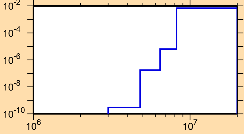
\sigma vs. E for ^{144}\text{Nd}(n,p)
