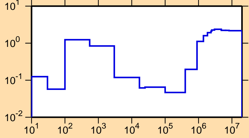
\sigma vs. E for ^{144}\text{Nd}(n,\text{nonel.})
