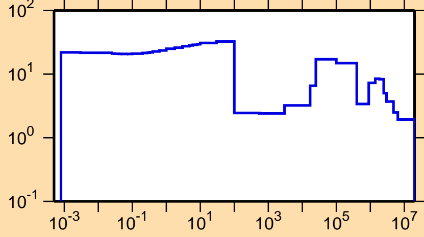
\Delta\sigma/\sigma vs. E for ^{144}\text{Nd}(n,\text{tot.})
