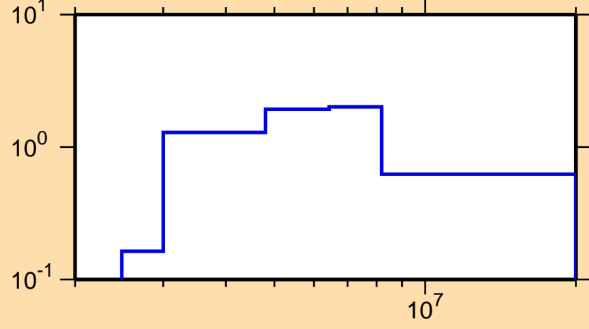
\sigma vs. E for ^{144}\text{Nd}(n,n\text{cont.})
