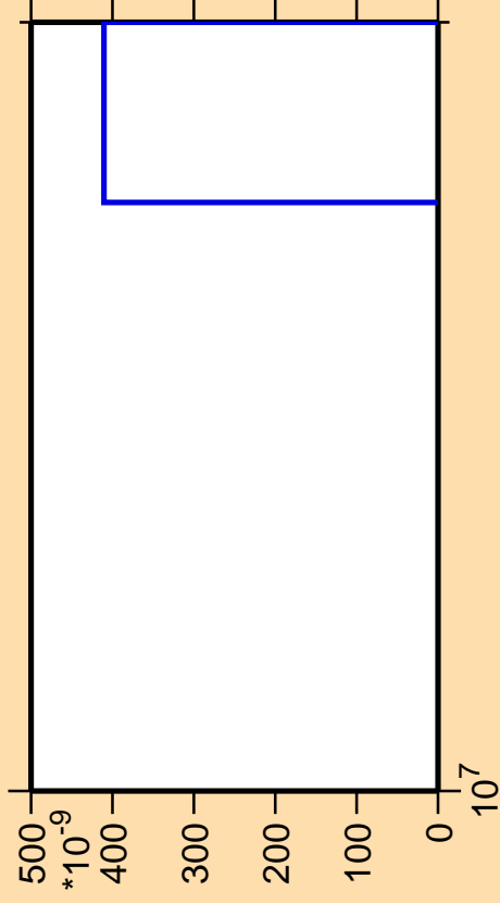
\Delta\sigma/\sigma vs. E for ^{147}\text{Nd}(\text{mt } 11)
