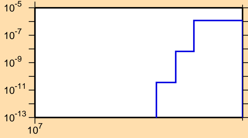
\sigma vs. E for ^{147}\text{Nd}(n,\text{nt})
