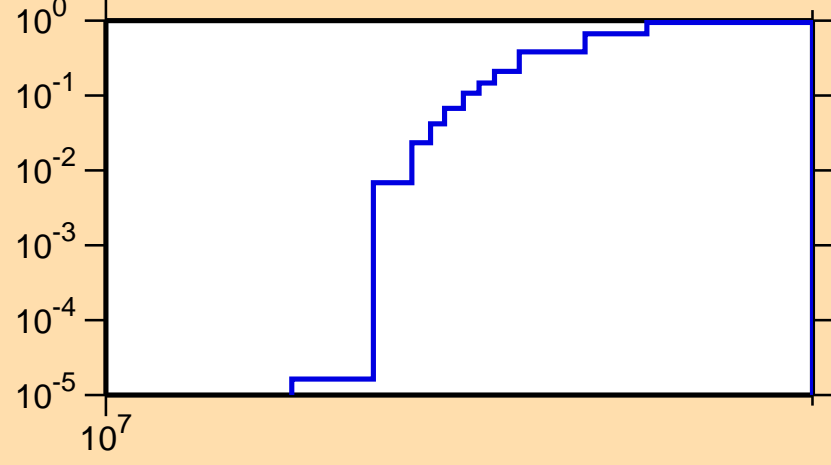
\sigma vs. E for ^{147}\text{Nd}(n,3n)
