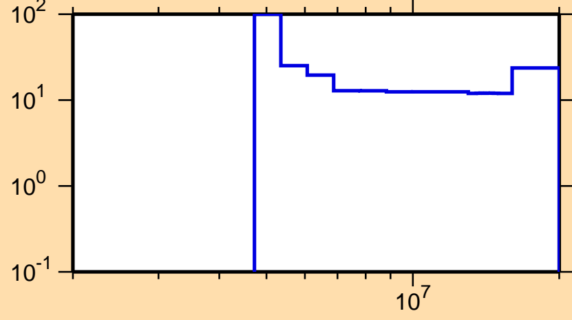
\Delta\sigma/\sigma vs. E for ^{147}\text{Nd}(n,2n)
