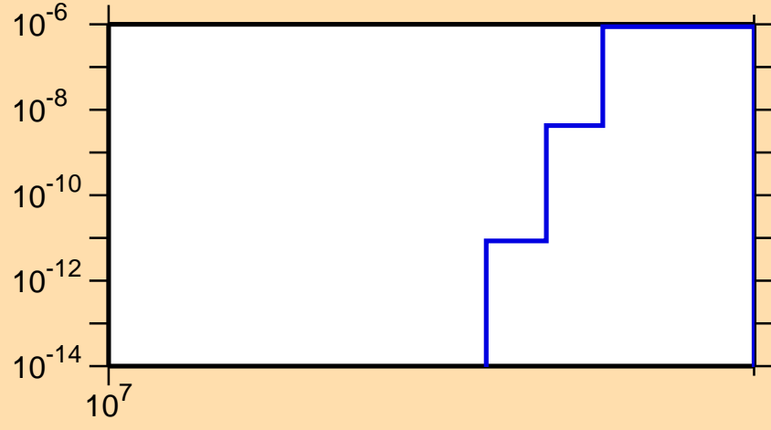
\sigma vs. E for ^{147}\text{Nd}(n,2np)
