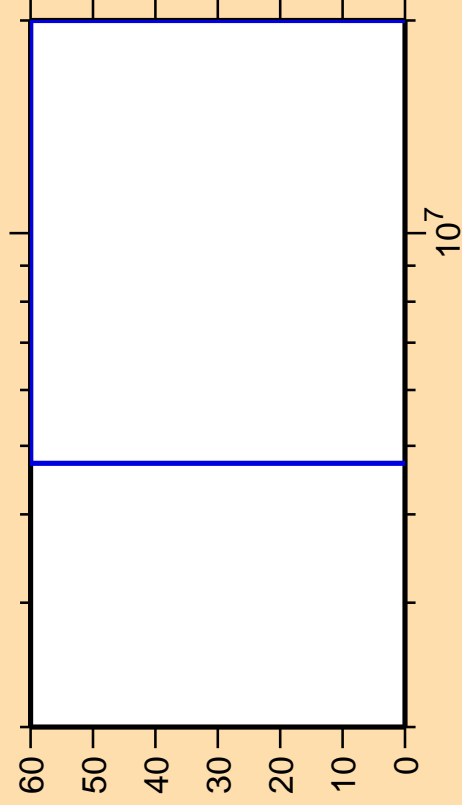
\Delta\sigma/\sigma vs. E for ^{147}\text{Nd}(n,\gamma)
