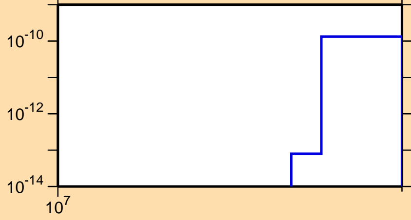
\sigma vs. E for ^{147}\text{Nd}(n,3n\alpha)
