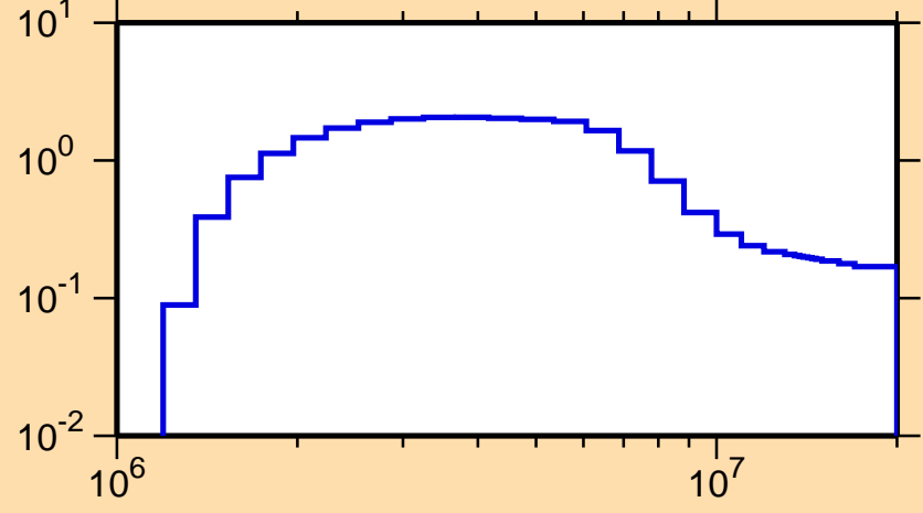
\sigma vs. E for ^{147}\text{Nd}(n,n\text{cont.})
