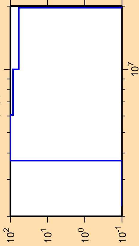
\Delta\sigma/\sigma vs. E for ^{147}\text{Nd}(n,p)
