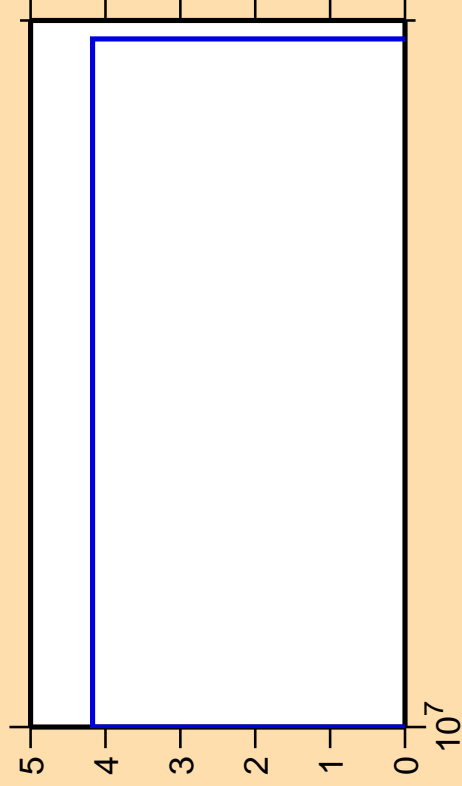
\Delta\sigma/\sigma vs. E for ^{147}\text{Nd}(n,3n\alpha)
