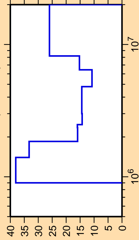
\Delta\sigma/\sigma vs. E for ^{147}\text{Nd}(n,ncont.)
