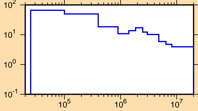
\Delta\sigma/\sigma vs. E for ^{147}\text{Nd}(n,\text{tot.})
