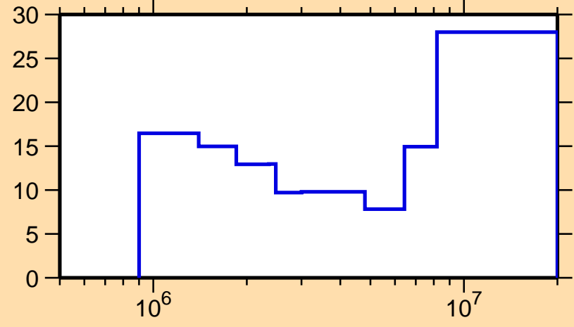
\Delta\sigma/\sigma vs. E for ^{147}\text{Nd}(n,inel.)
