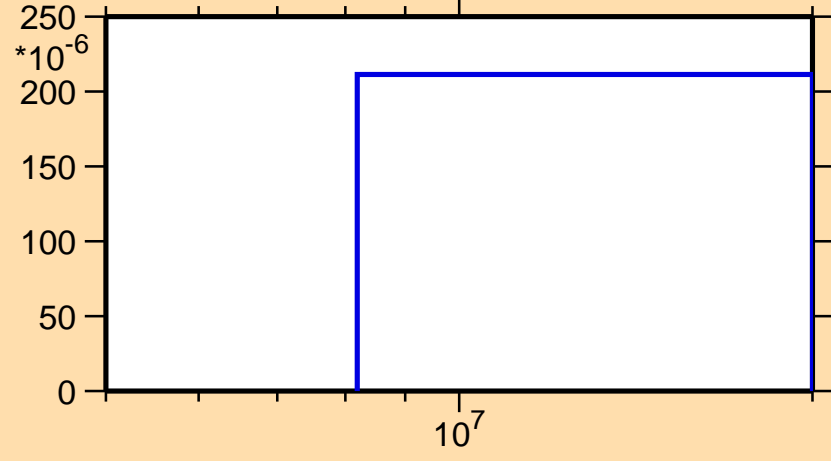
\sigma vs. E for ^{147}\text{Nd}(n,t)
