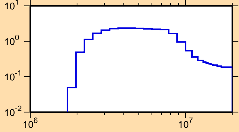
\sigma vs. E for ^{148}\text{Nd}(n,n\text{cont.})
