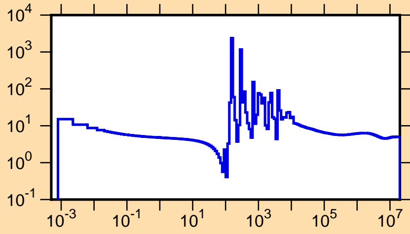
\sigma vs. E for ^{148}\text{Nd}(n,\text{tot.})
