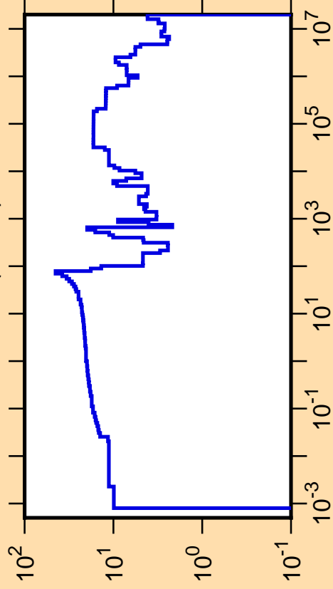
\Delta\sigma/\sigma vs. E for ^{148}\text{Nd}(n,\text{tot.})
