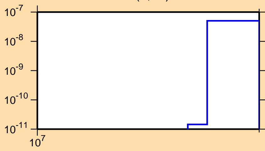
\sigma vs. E for ^{148}\text{Nd}(n,\text{nd})
